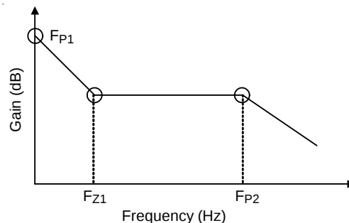
Figure 5. Bode Plot of the Type-II Compensation
