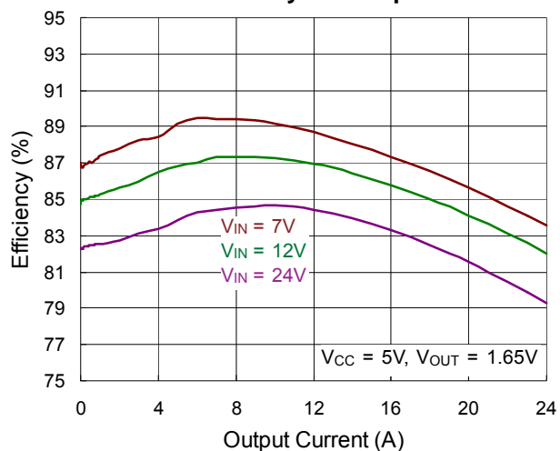
V1P65 Efficiency vs. Output Current
