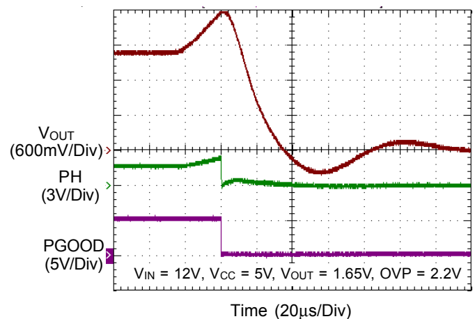
Over-Voltage Protection
