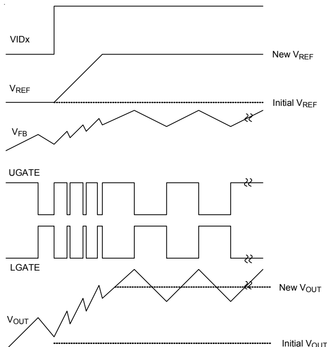
Figure 3. Upward Transition of Output Voltage
