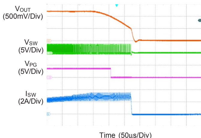
Figure 2. Over-Current Protection
