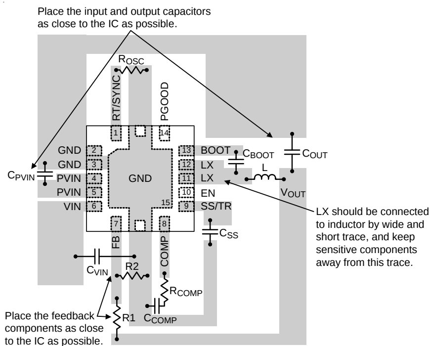
Figure 11. PCB Layout Guide
