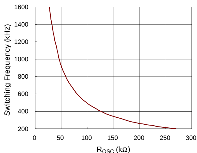
Figure 7. Switching Frequency vs. R_{OSC} Resistor
