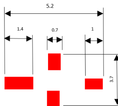
PCB Footprint
