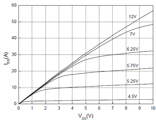
Figure 2. Typical Output Characteristics T_J=150^\circ\text{C}
