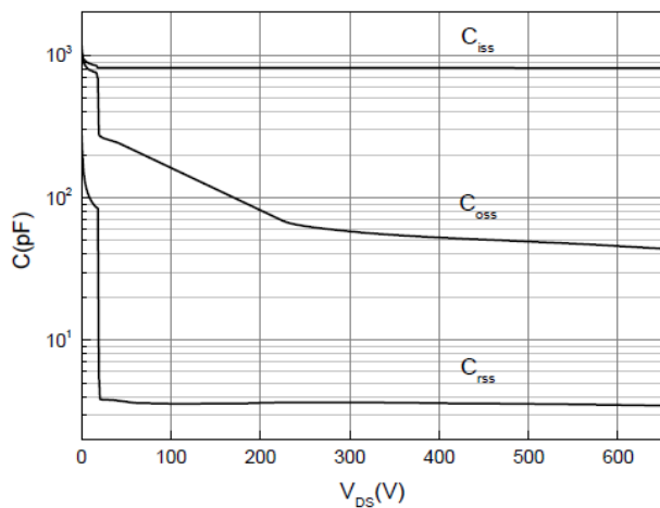
Figure 5. Typical Capacitance
