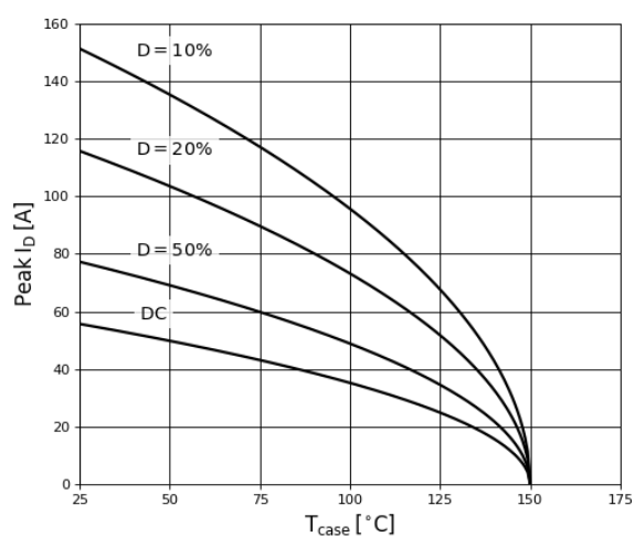
Figure 12. Current Derating
