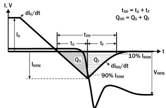
Figure 20. Diode Recovery Waveform
