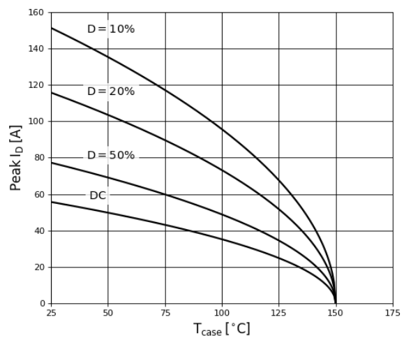
Figure 11. Current Derating
