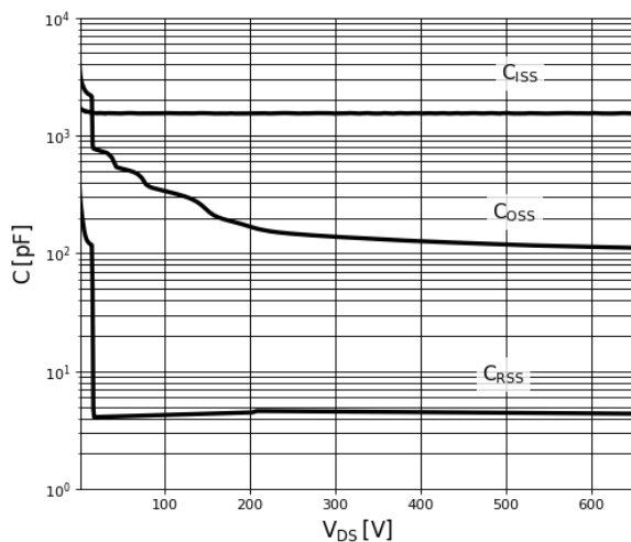
Figure 6. Typical Capacitance
