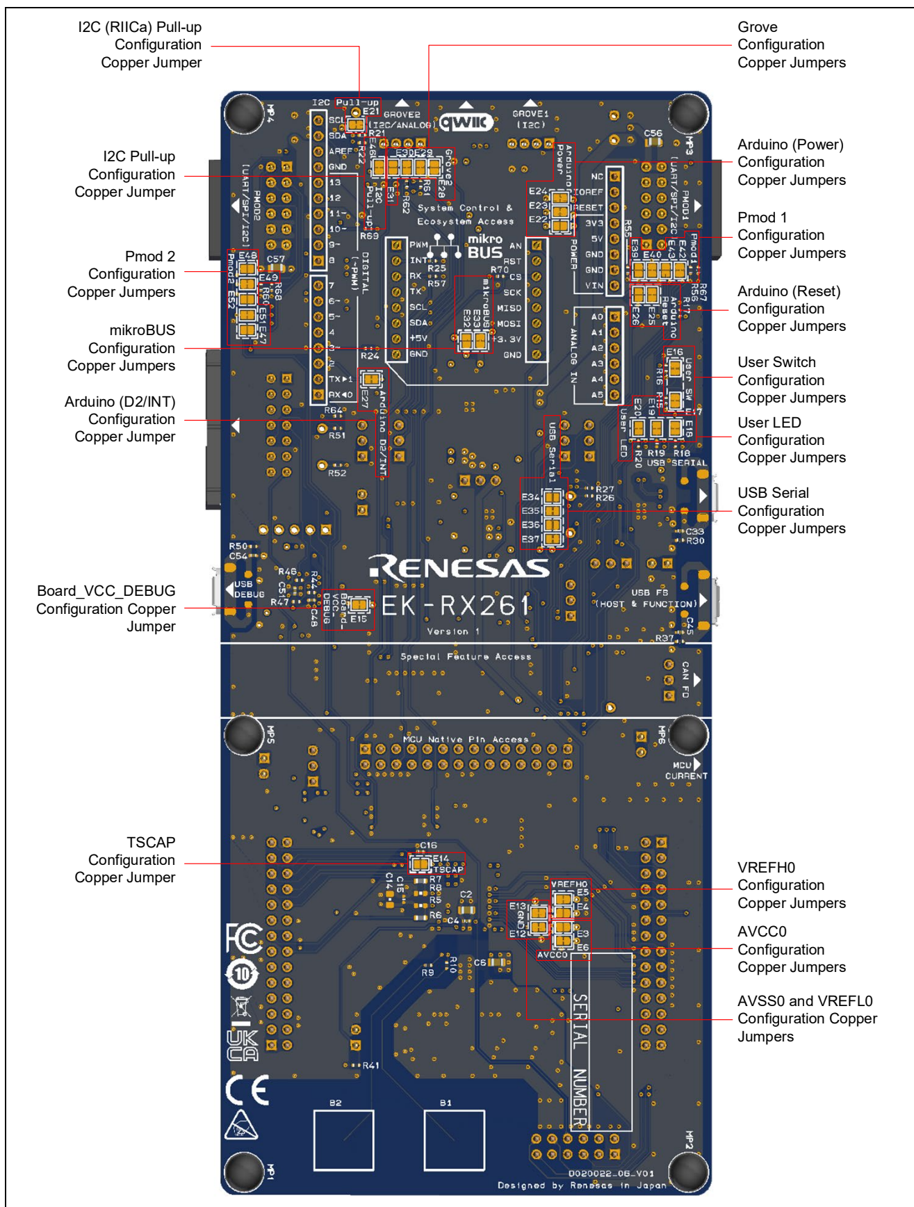
Figure 2. EK-RX261 v1 Bottom Side
