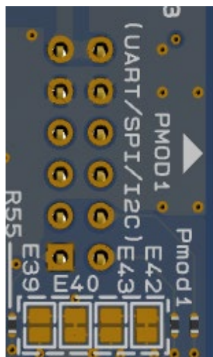
Figure 16. Pmod 1 Copper jumpers (bottom side)
