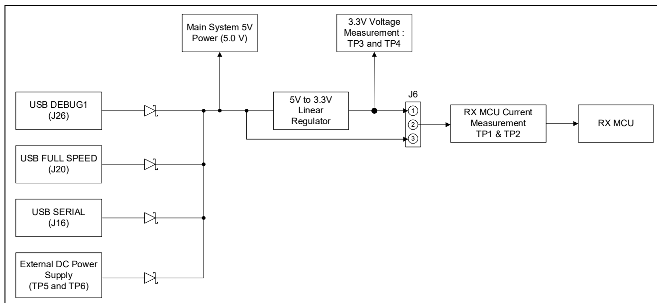
Figure 11. Power Supply
