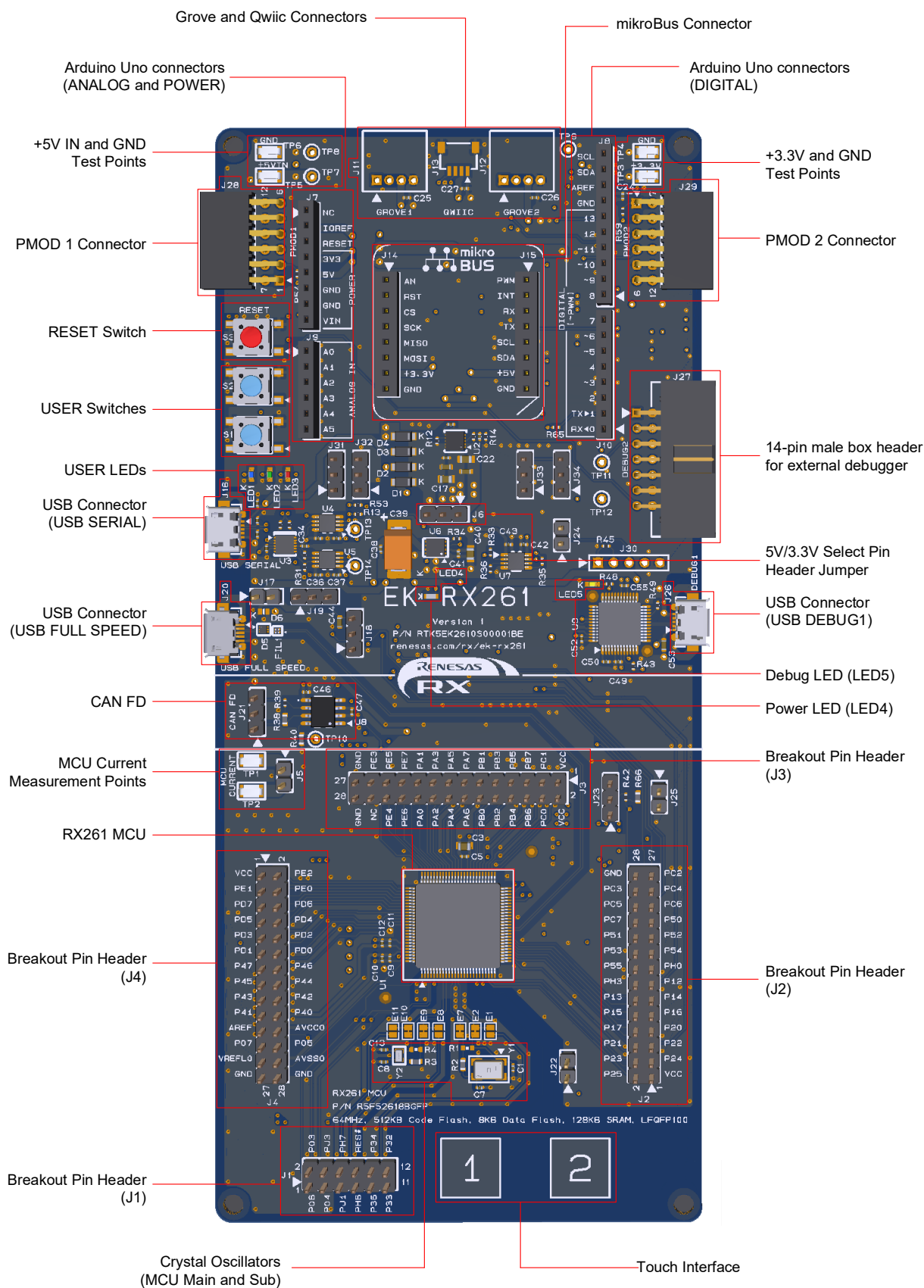
Figure 1. EK-RX261 v1 Top Side
