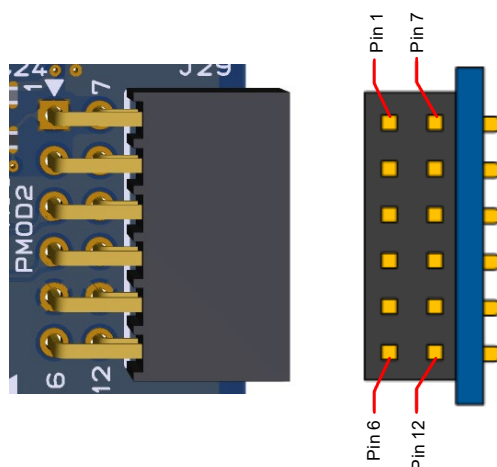
Figure 17. Pmod 2 connector
