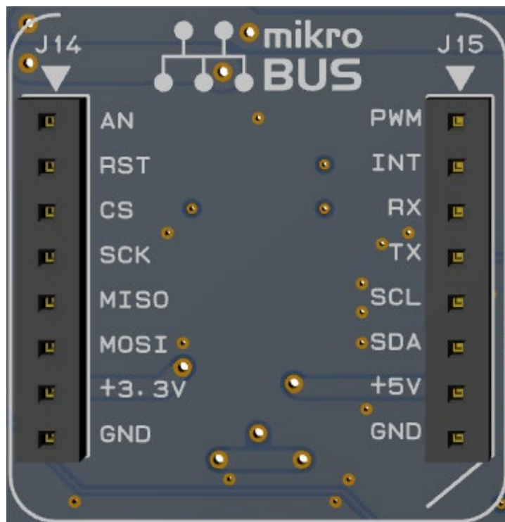
Figure 22. mikroBUS Connectors
