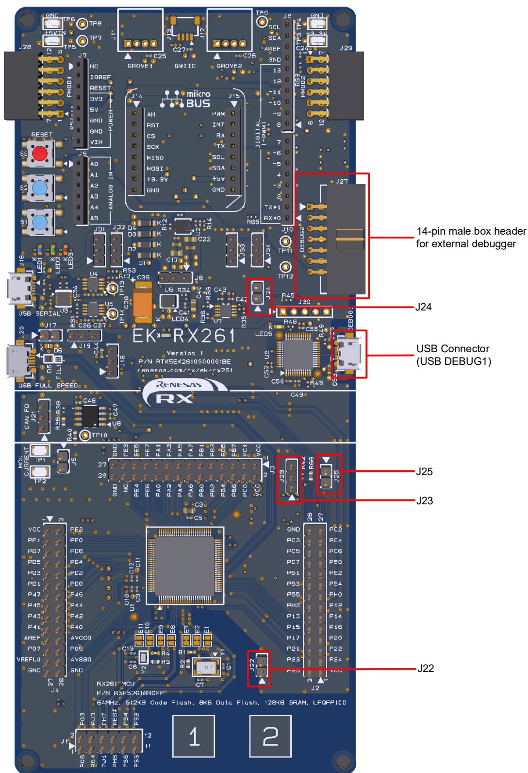
Figure 12. EK-RX261 v1 Debug Interface
