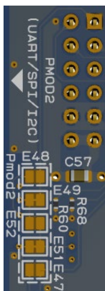
Figure 19. Pmod 2 Copper jumpers (bottom side)
