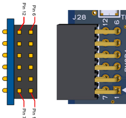
Figure 14. Pmod 1 connector
