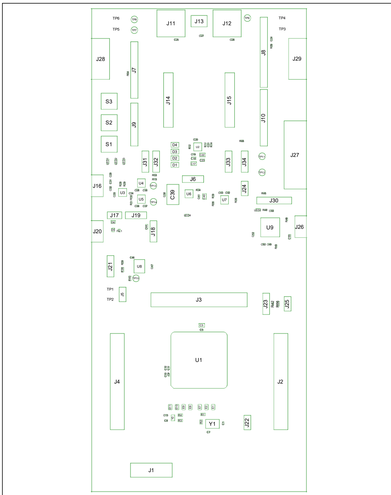
Figure 6. Reference number for components on the EK-RX261 v1 (top side)
