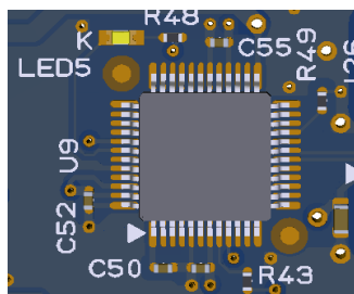
Figure 28. Debug LED
