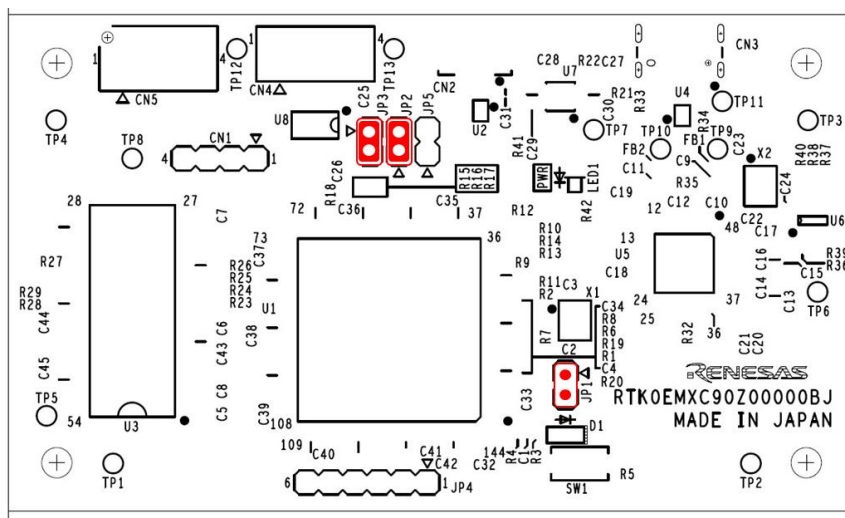
Figure 4-8 Default jumper pin setting of Communication board
