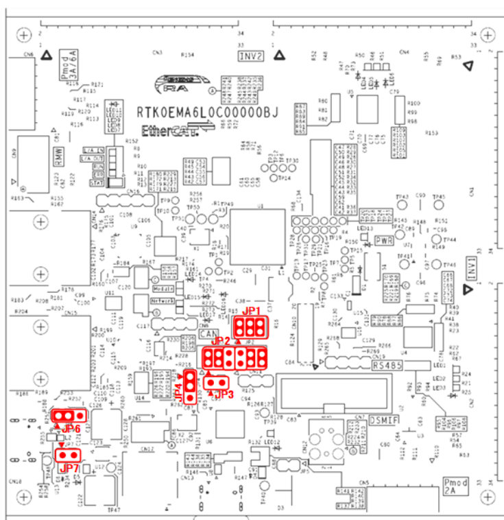
Figure 4-7 Default jumper pin setting of CPU board
