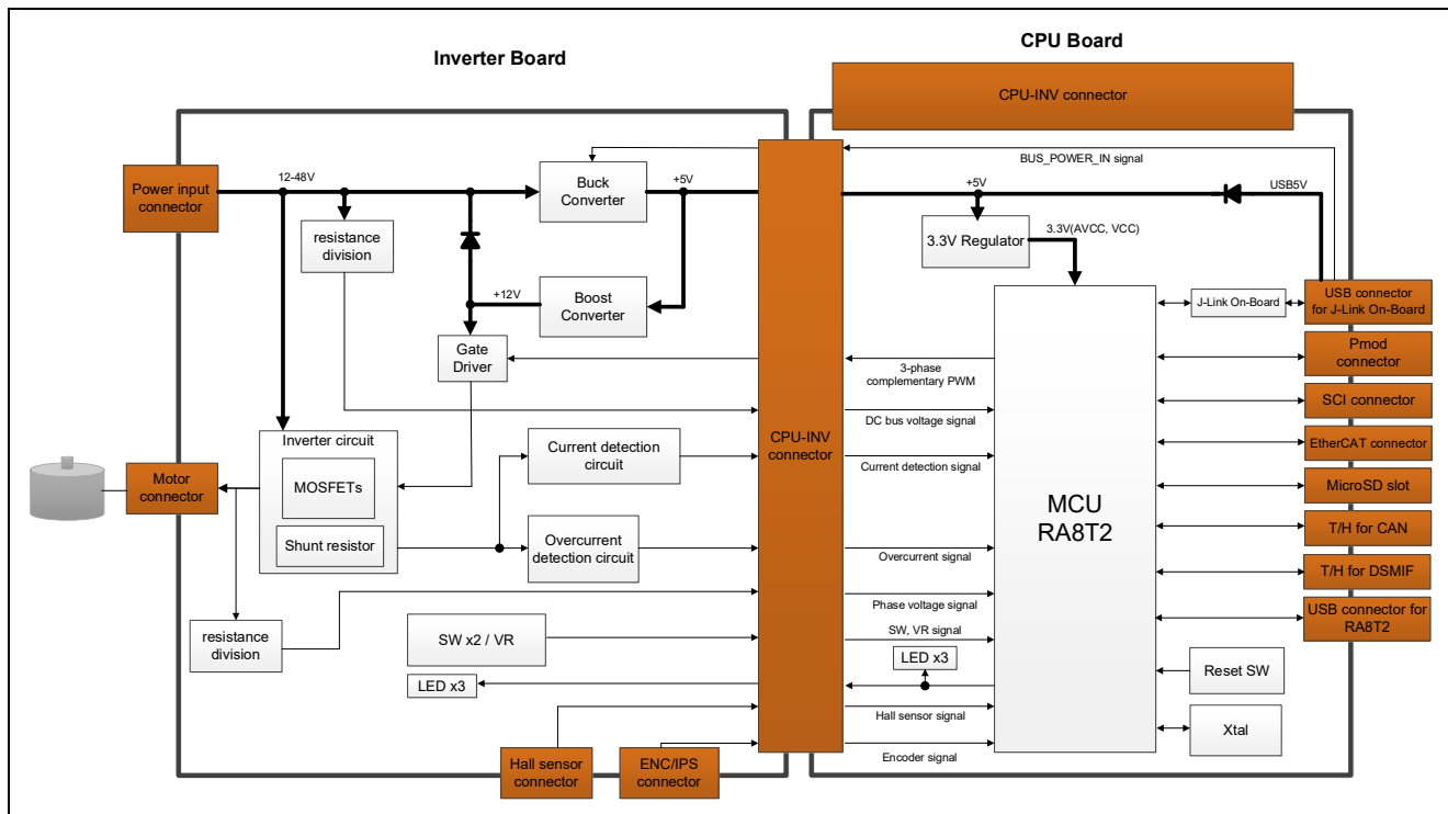
Figure 4-1 MCK-RA8T2 block diagram
