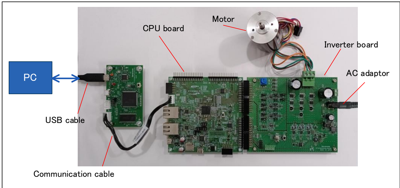
Figure 4-9 Board connection
