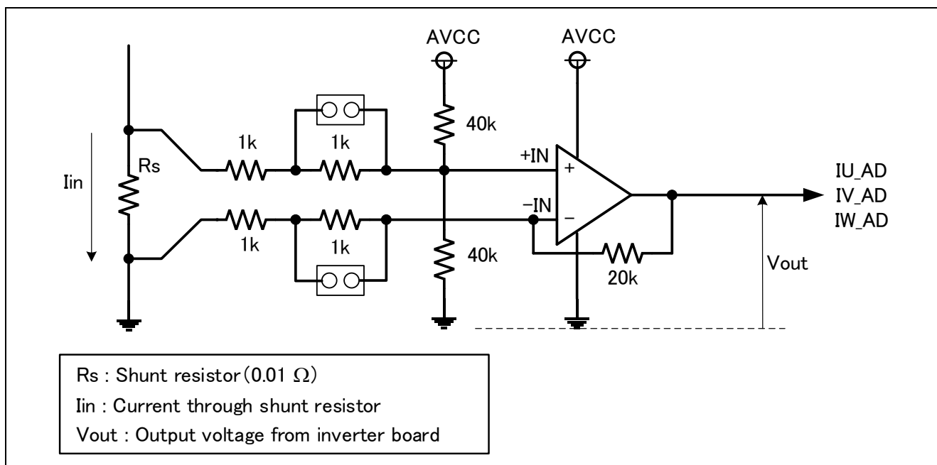
Figure 5-2 Current detection circuit
