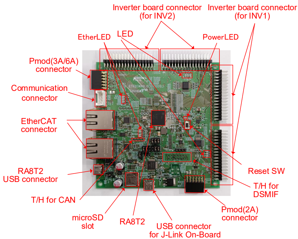
Figure 4-3 CPU board layout
