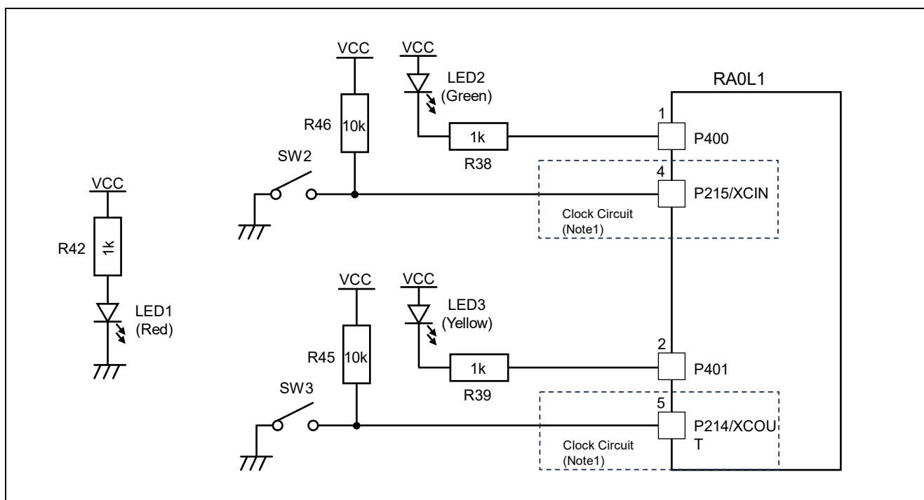
Figure 9 Push Switch and LED Circuits
