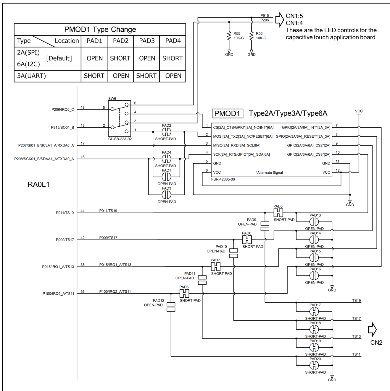
Figure 10 PMOD1 Interface Switching Circuit
