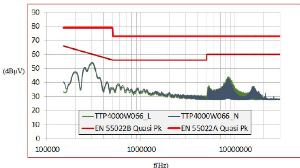
Figure 14. Conducted Emissions at 115V, 1150W
