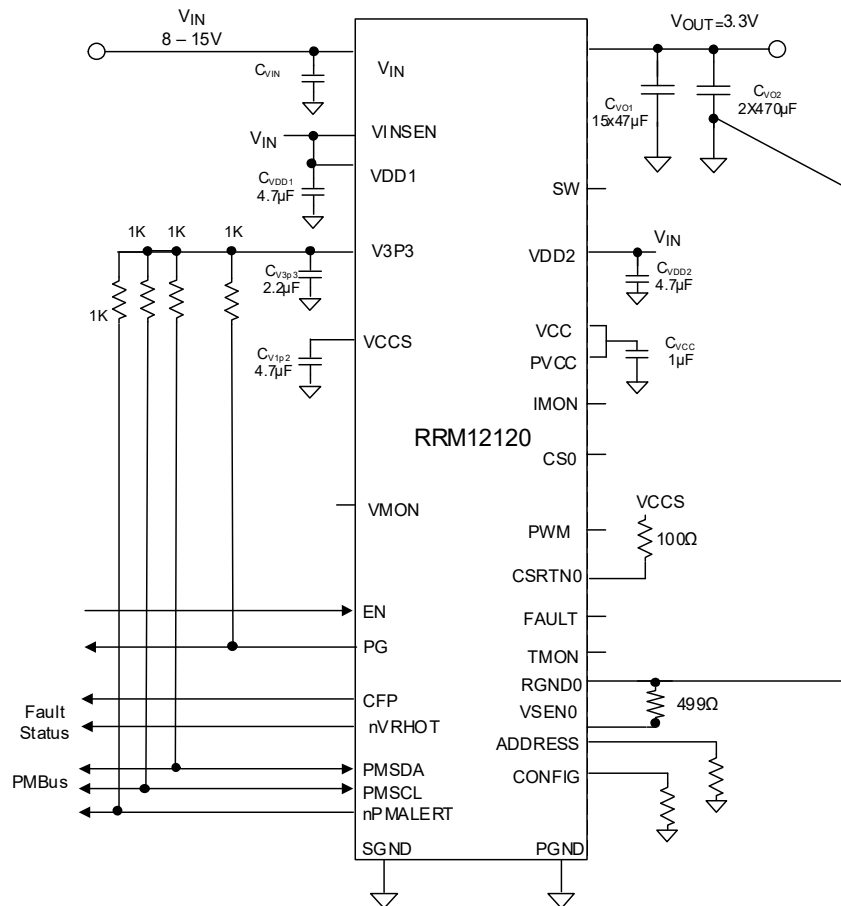
Figure 5. Typical Application Circuit for 3.3V Output, 20A Load
