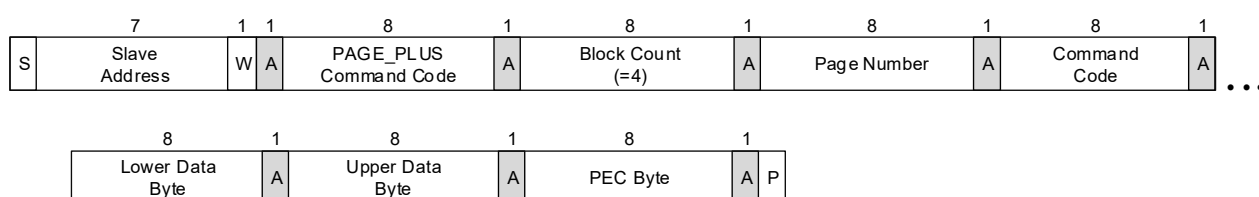
Figure 47. PAGE_PLUS_WRITE Command with a PEC Byte
