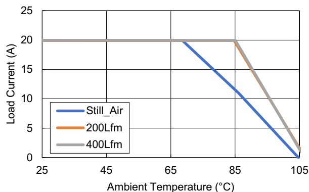
Figure 31. Thermal Derating Curve, V_{IN} = 12V , V_{OUT} = 3.3V , f_{SW} = 700kHz
