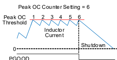
Figure 35. Peak OC Operation
