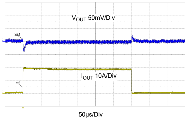
Figure 20. Transient Response, V_{IN} = 12V , V_{OUT} = 3.3V , 0A to 20A to 0A, 5A/μs Step Load, C_{OUT} = 15 \times 47\mu F Ceramic + 2 \times 470\mu F Polymer Capacitor
