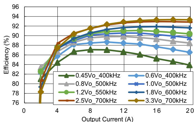
Figure 7. Efficiency vs Load Current at V_{IN} = 12V , with External 5V and 3.3V Supply
