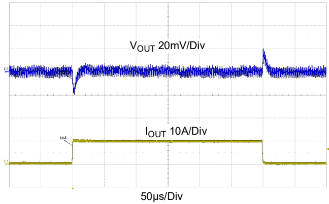
Figure 19. Transient Response, V_{IN} = 12V , V_{OUT} = 1.8V , 0A to 10A to 0A, 5A/μs Step Load, C_{OUT} = 7 \times 47\mu F Ceramic + 2 \times 470\mu F Polymer Capacitor
