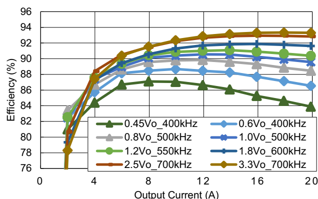
Figure 1. Efficiency vs Load Current at V_{IN} = 12V, with External 5V and 3.3V Supply
