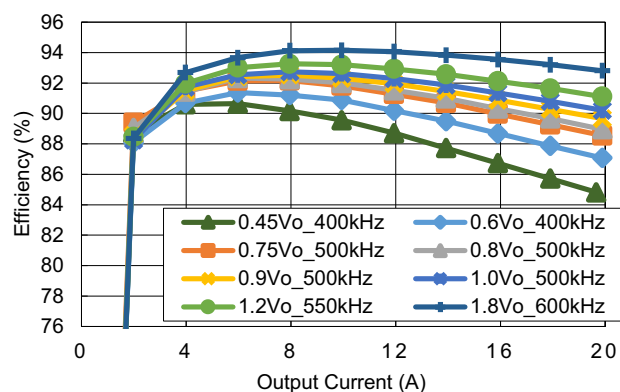
Figure 9. Efficiency vs Load Current at V_{IN} = 5V , with External 5V and 3.3V Supply
