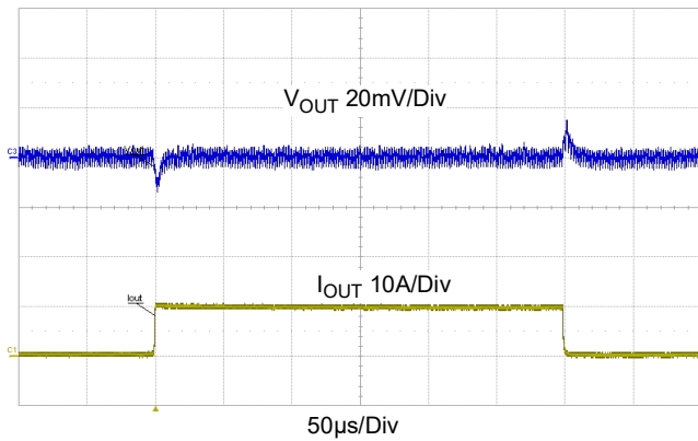
Figure 18. Transient Response, V_{IN} = 12V , V_{OUT} = 1.2V , 0A to 10A to 0A, 5A/μs Step Load, C_{OUT} = 7 \times 47\mu F Ceramic + 2 \times 470\mu F Polymer Capacitor
