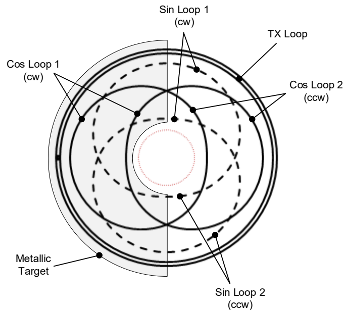
Figure 8. Coil Design for a 360° Rotary Sensor
