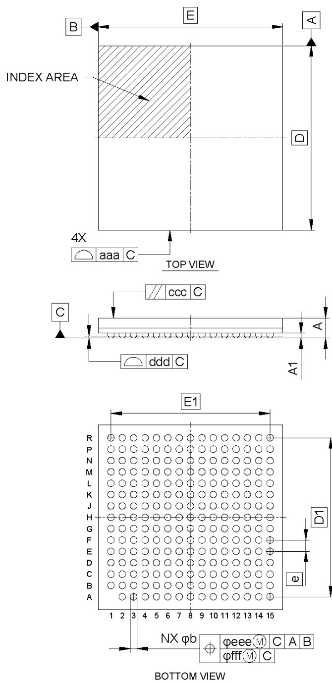
Figure 2.1 BGA 224-pin
