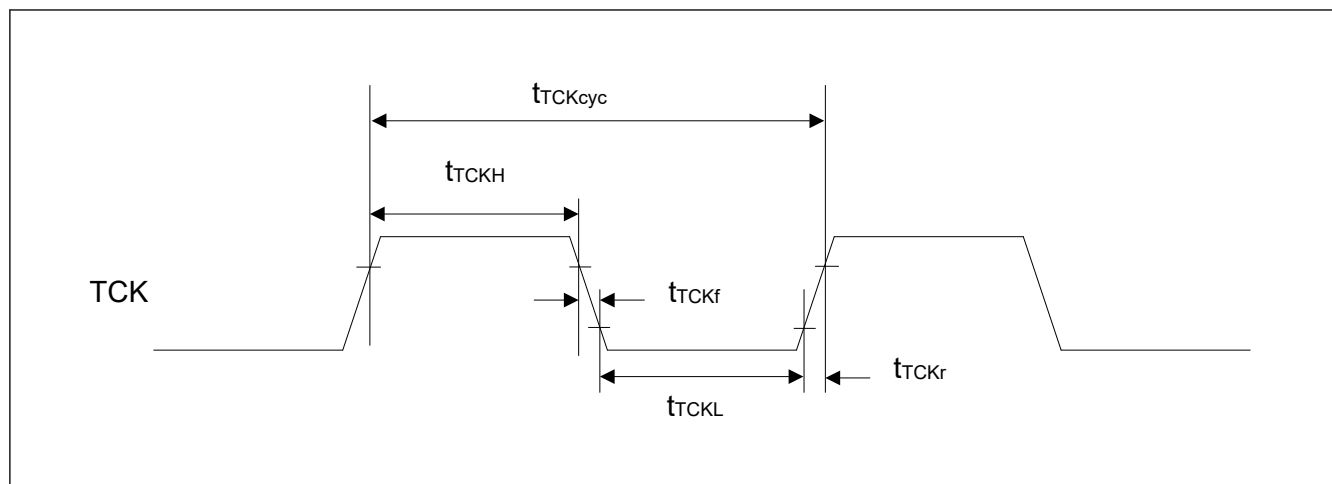
Figure 2.96 JTAG TCK timing
