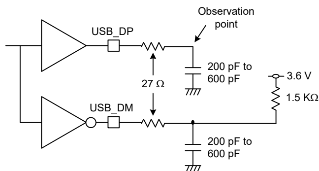
Figure 2.81 Test circuit in low-speed mode
