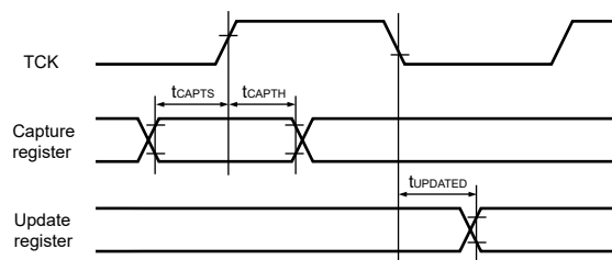
Figure 2.94 Boundary scan input/output timing (2)
