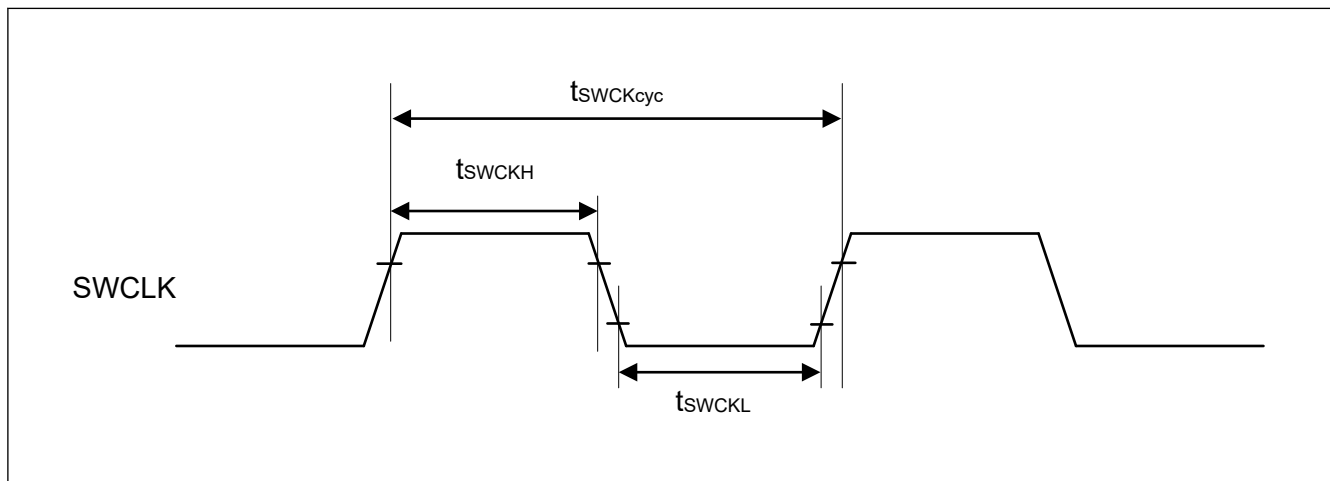
Figure 2.98 SWD SWCLK timing
