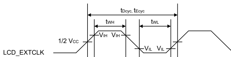
Figure 2.76 LCD_EXTCLK clock timing
