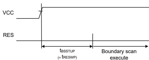
Figure 2.95 Boundary scan circuit startup timing
