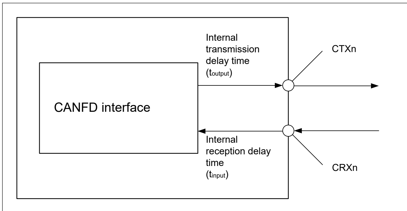
Figure 2.79 CANFD interface condition
