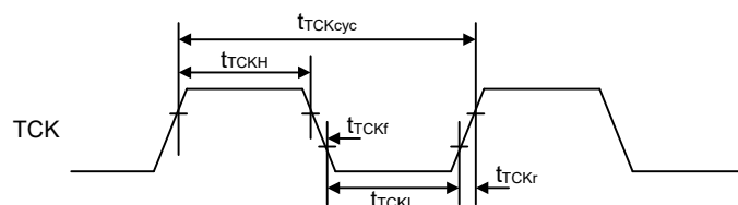
Figure 2.92 Boundary scan TCK timing
