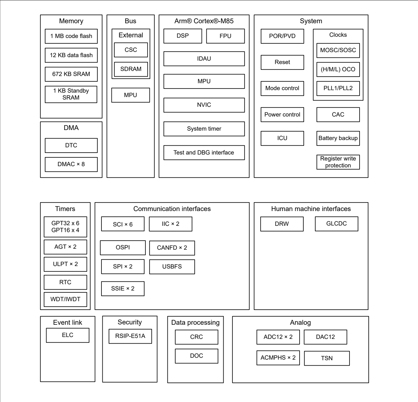
Figure 1.1 Block diagram
