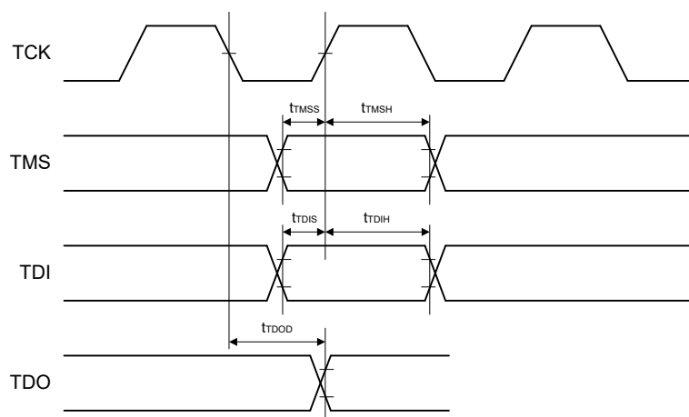
Figure 2.93 Boundary scan input/output timing (1)
