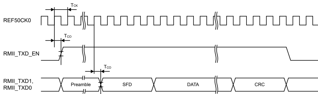
Figure 2.62 RMII transmission timing
