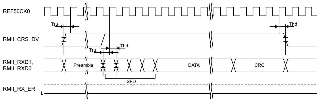
Figure 2.63 RMII reception timing in normal operation
