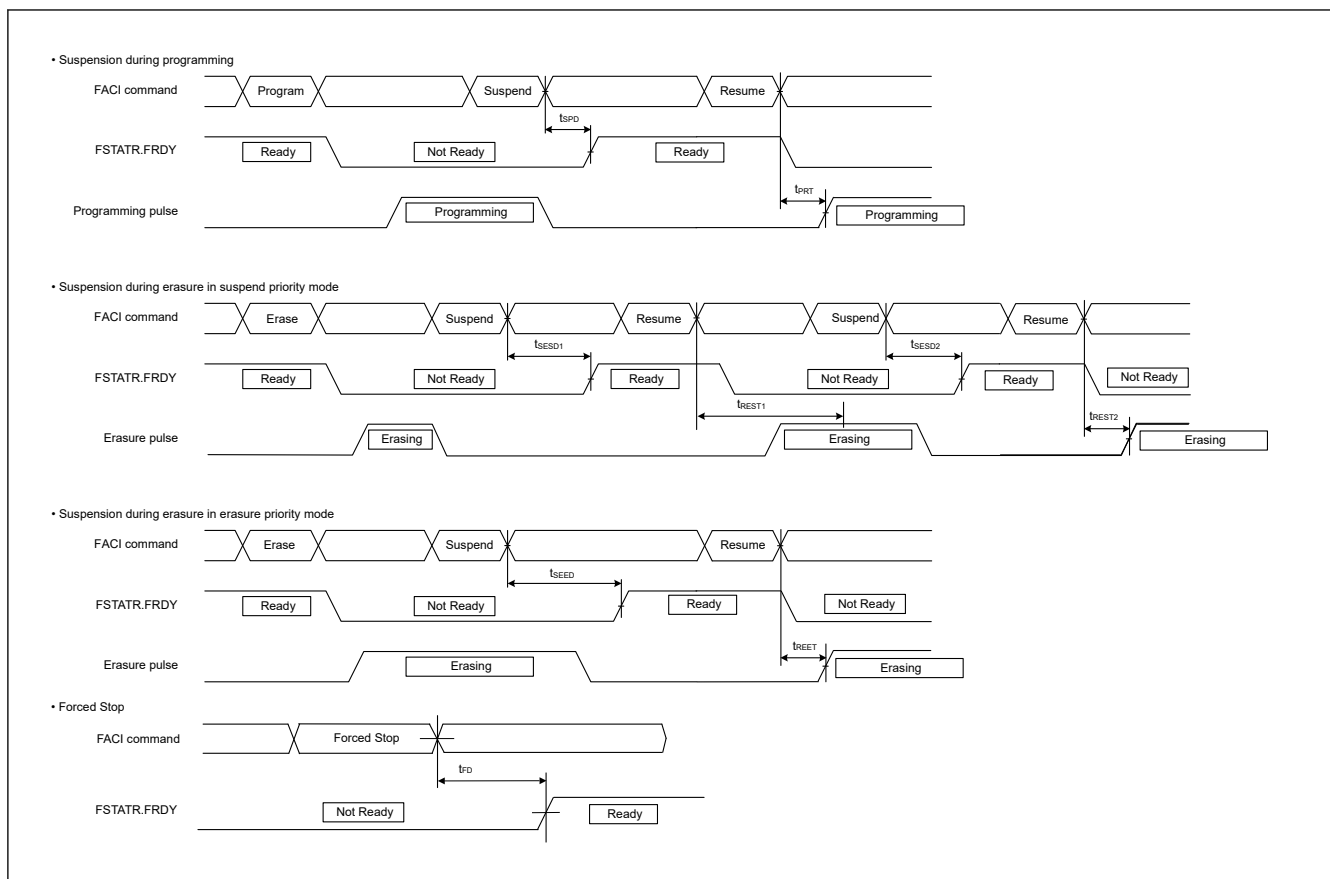
Figure 2.85 Suspension and forced stop timing for flash memory programming and erasure
