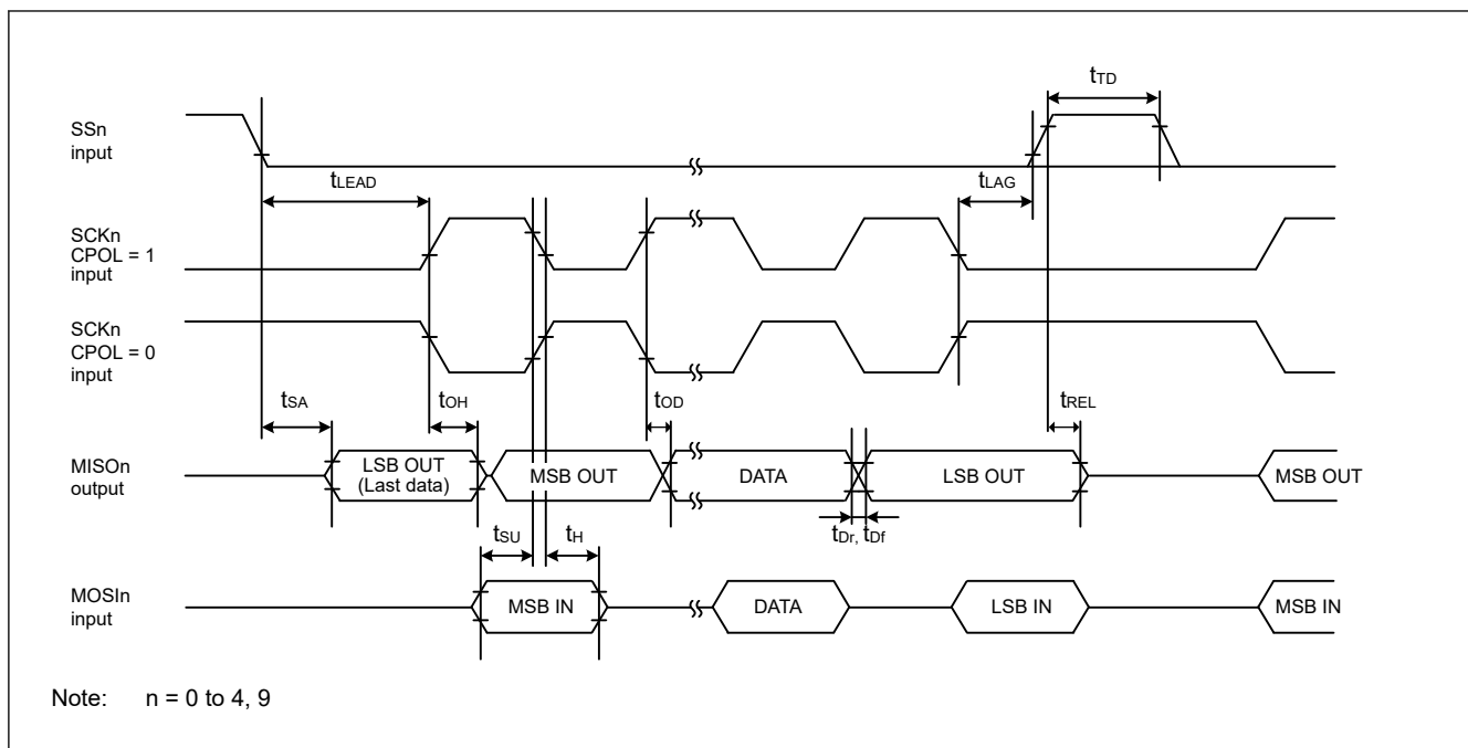
Figure 2.40 SCI simple SPI mode timing for slave when CPHA = 1
