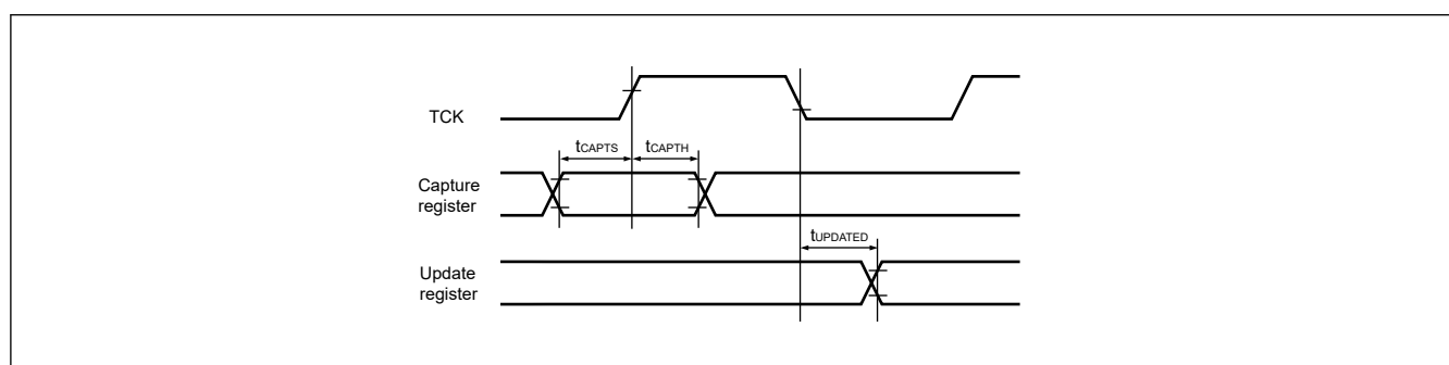
Figure 2.88 Boundary scan input/output timing (2)
