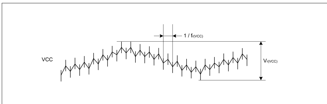
Figure 2.2 Ripple waveform
