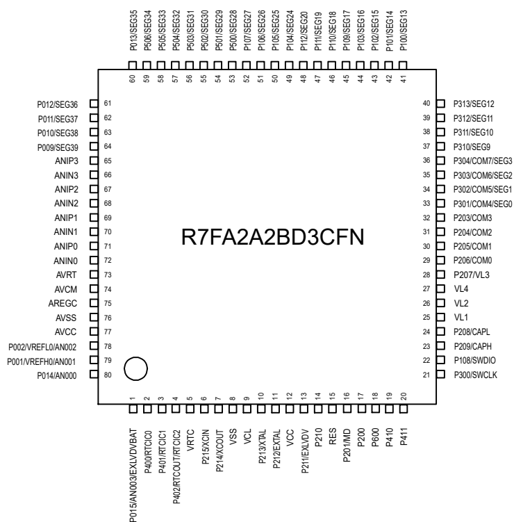
Figure 1.5 Pin assignment for LQFP 80-pin (top view)
