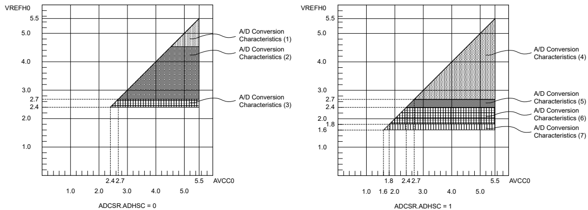
Figure 2.37 AVCC to VREFH0 voltage range
