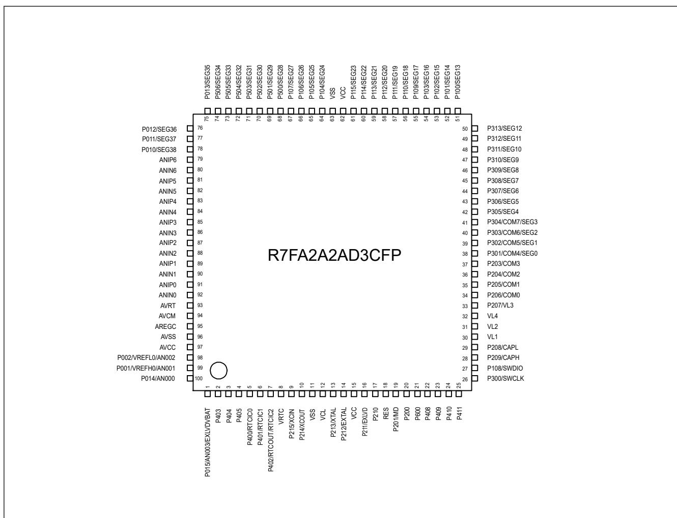
Figure 1.3 Pin assignment for LQFP 100-pin 7 ch (top view)
