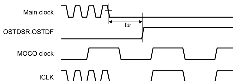
Figure 2.41 Oscillation stop detection timing
