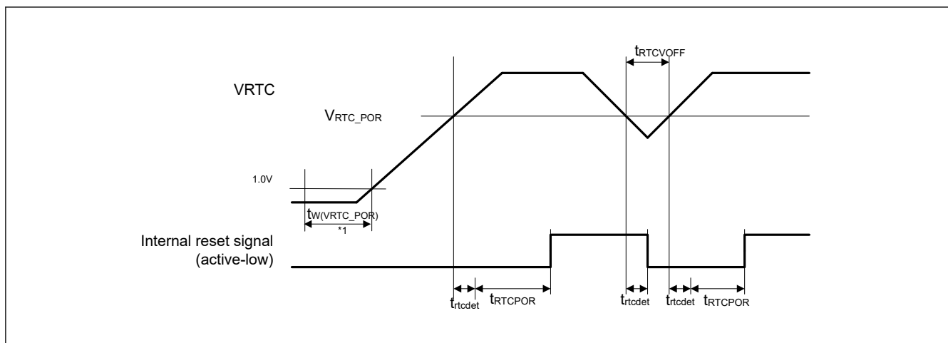
Figure 2.47 Voltage detection reset timing and power-on reset timing of VRTC
