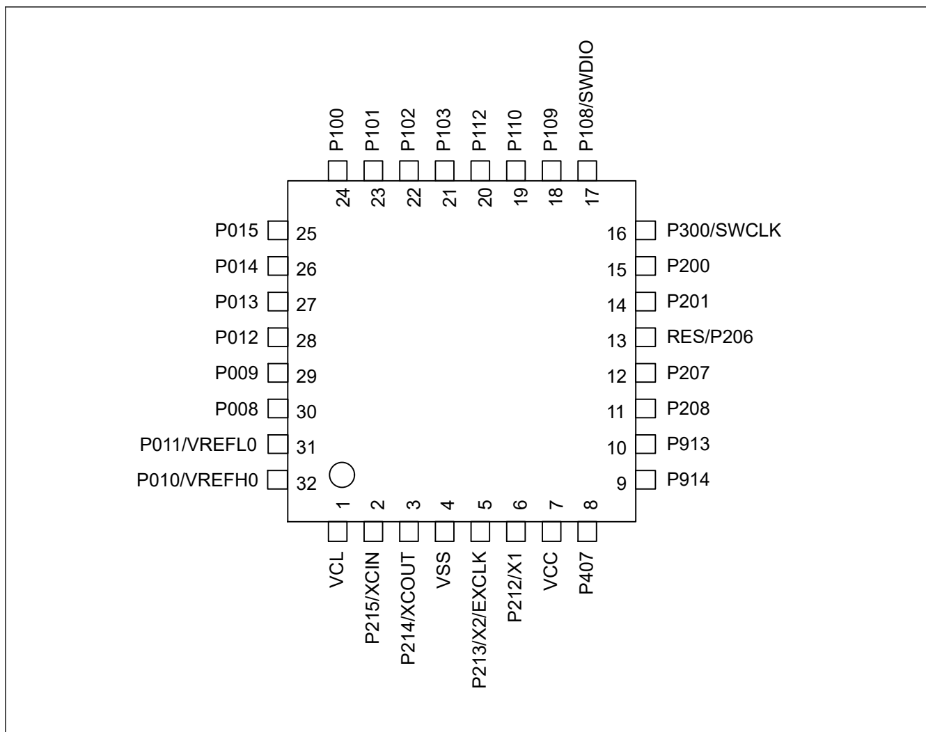
Figure 1.4 Pin assignment for LQFP / HWQFN 32-pin (top view)
