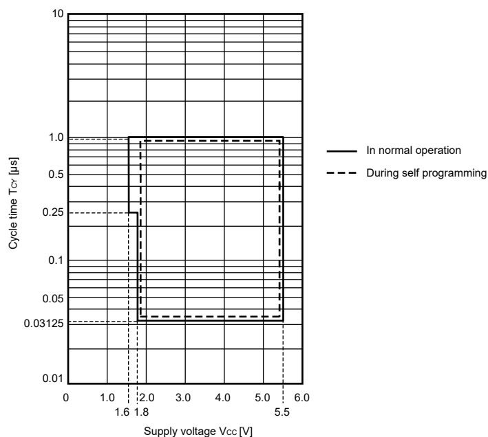
Figure 2.2 T cy vs V cc in High-speed mode
