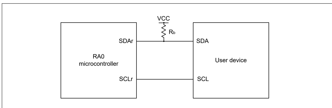
Figure 2.19 Connection in the simplified IIC communications with devices operating at the same voltage levels
