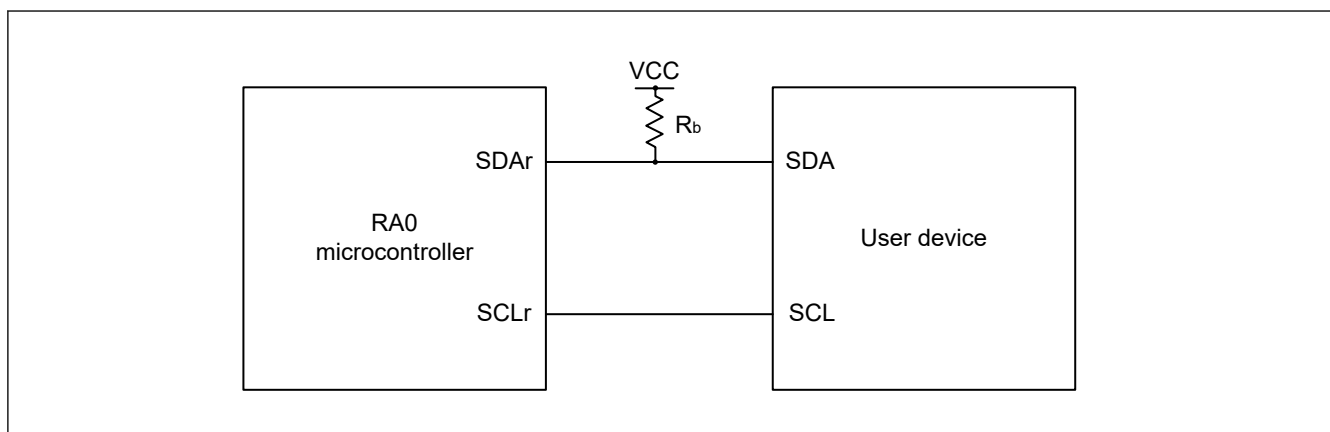
Figure 2.19 Connection in the simplified IIC communications with devices operating at same voltage levels
