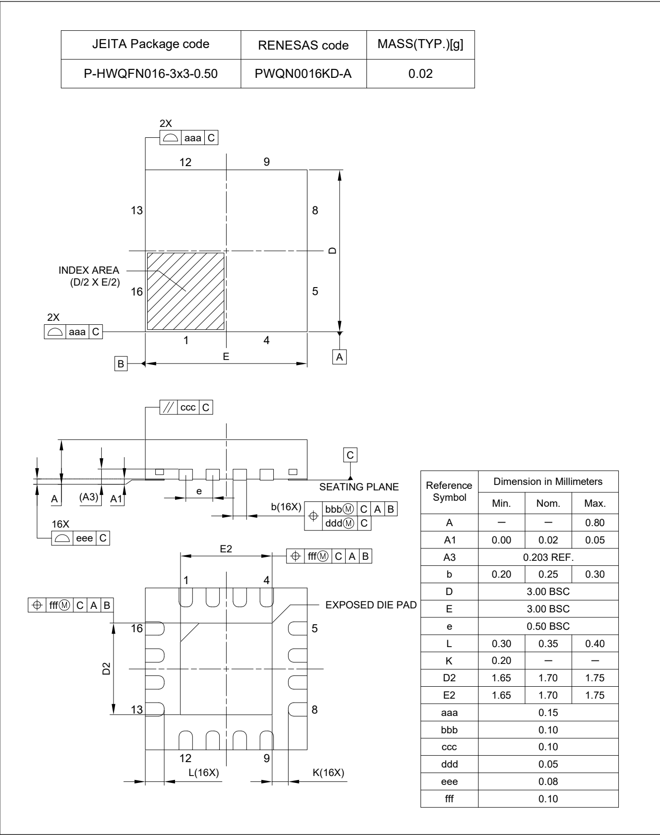
Figure A2.5 HWQFN 16-pin
