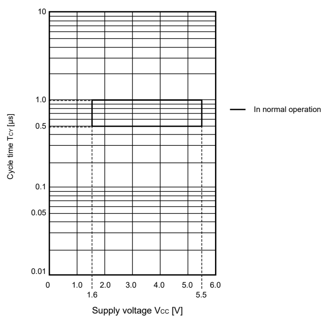
Figure 2.4 T_{CY} vs V_{CC} in Low-speed mode
