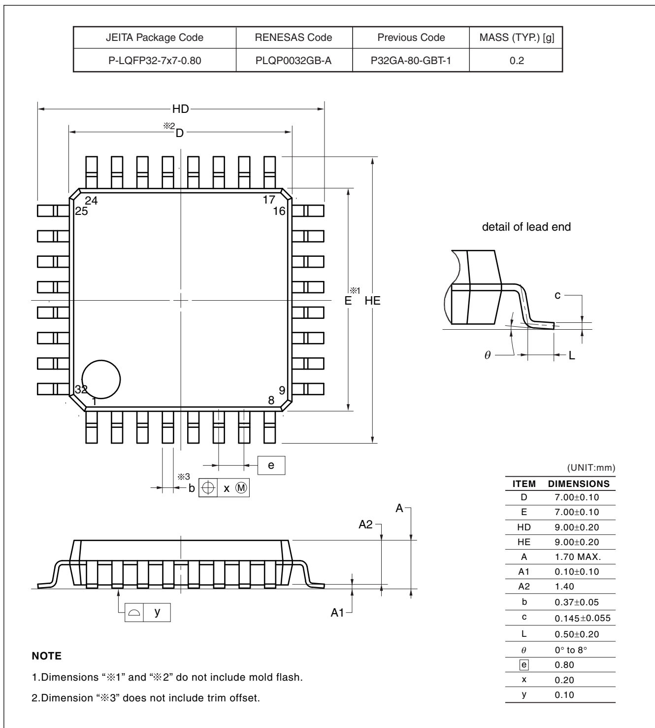
Figure A2.1 LQFP 32-pin
