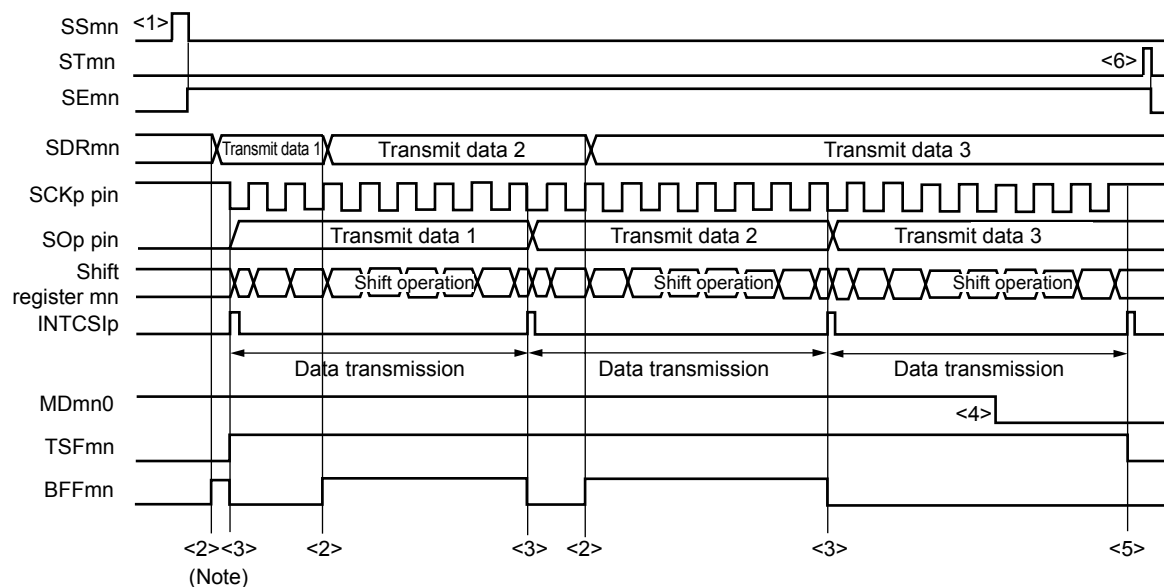
<R> Figure 14-31. Timing Chart of Master Transmission (in Continuous Transmission Mode) (Type 1: DAPmn = 0, CKPmn = 0)
