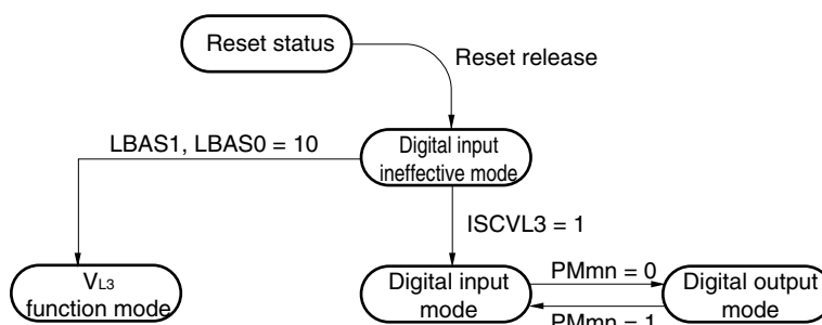
Figure 4-49. V L3 /P125 Pin Function Status Transition Diagram
