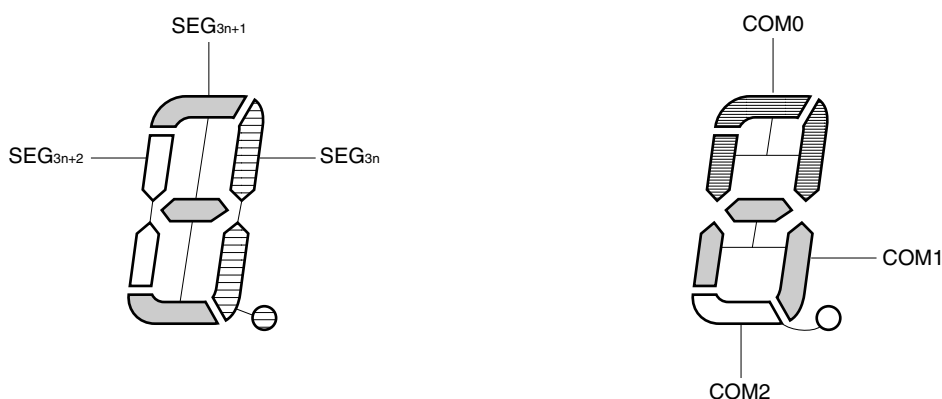
Figure 17-31. Three-Time-Slice LCD Display Pattern and Electrode Connections
