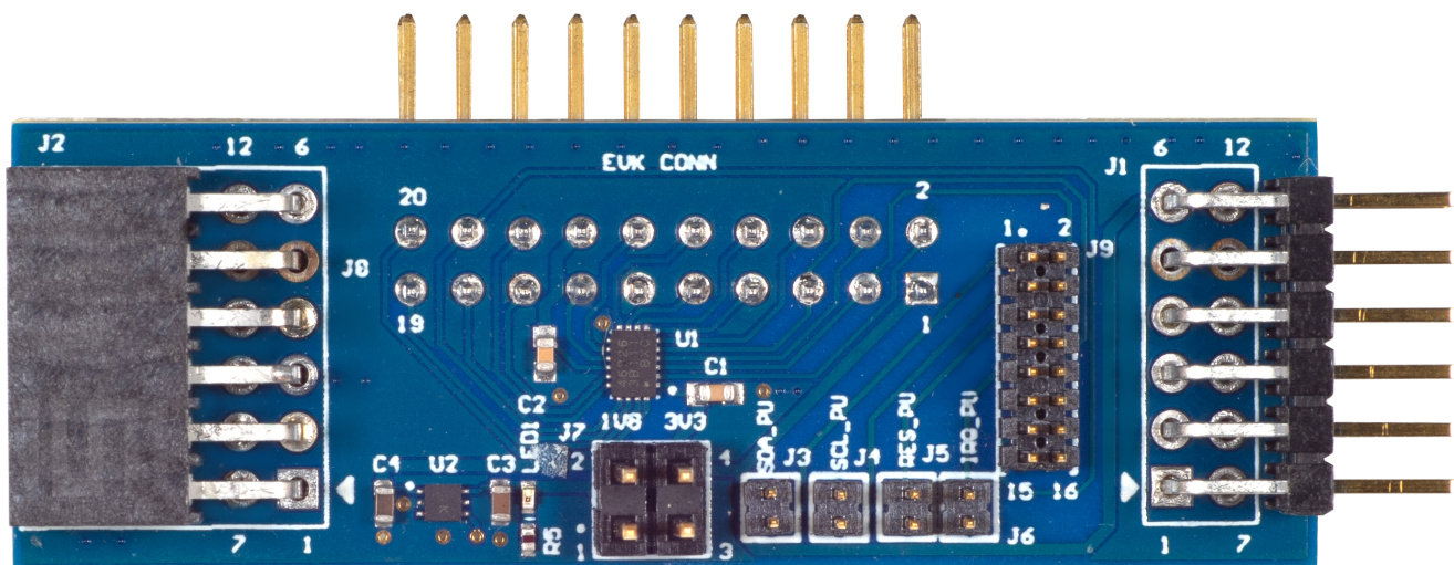
Figure 1. QCIOT-SLG46826POCZ Board
