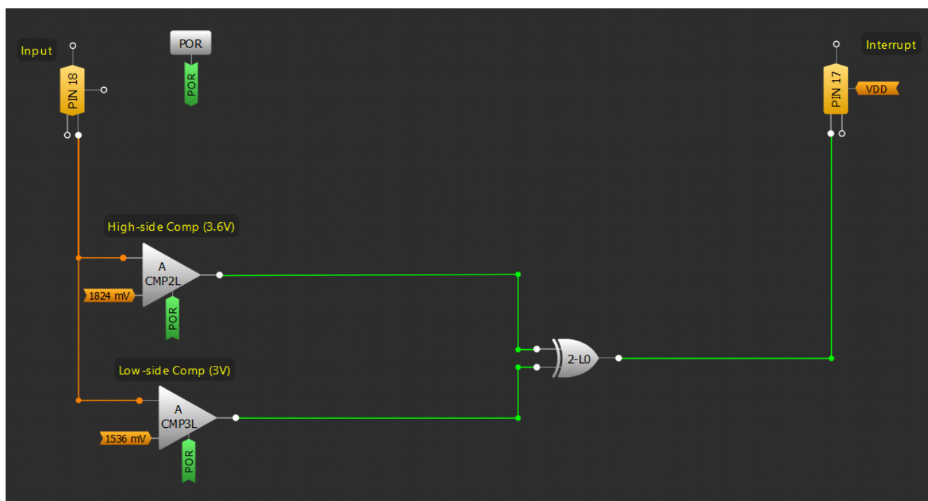
Figure 16. Window Comparator Schematic
