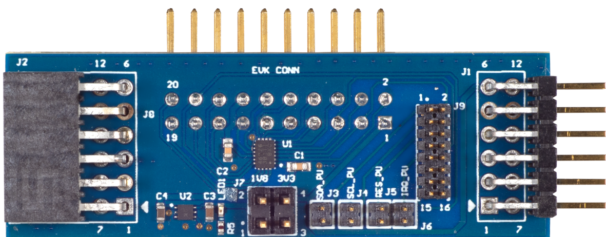
Figure 5. QCIOT-SLG46826POCZ Board (Top)
