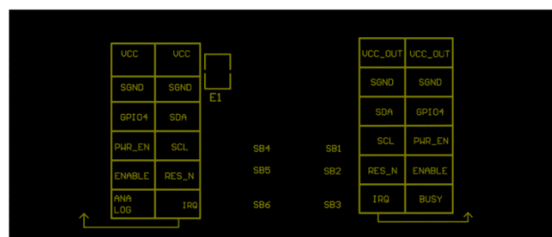
Figure 18. Bottom Overlay
