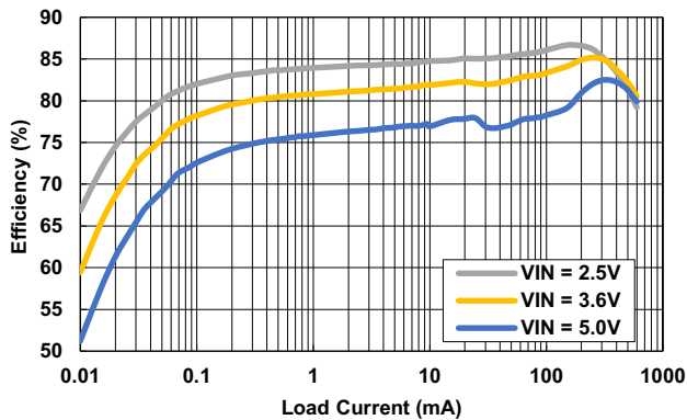
Figure 5. Efficiency vs Load Current: V_{OUT} = 0.8V
