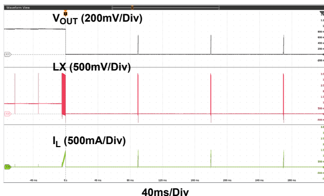
Figure 29. Output Short-Circuit Behavior (Hiccup Mode)
