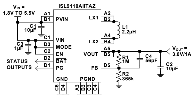
FIGURE 28. TYPICAL ISL9110A IITAZ APPLICATION
