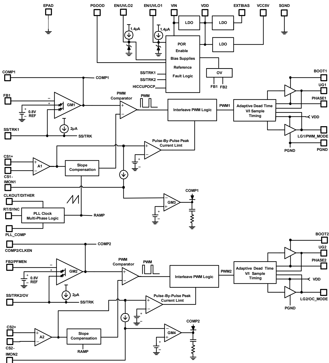
Figure 5. Block Diagram
