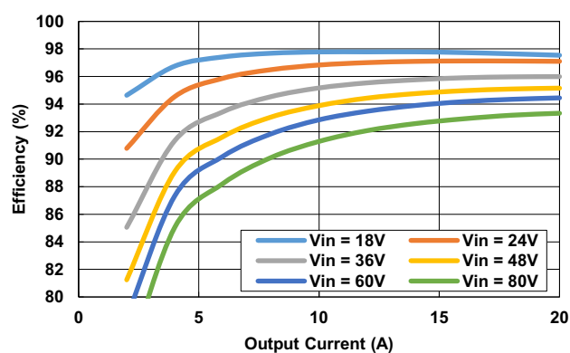
Figure 19. CCM Mode Efficiency
