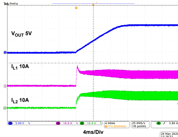
Figure 27. Dual-Phase Waveforms, Start-Up Waveform, V_{IN} = 48V I_O = 20A , CCM
