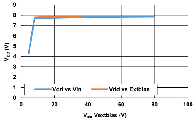
Figure 9. V DD Line Regulation at 20mA Load
