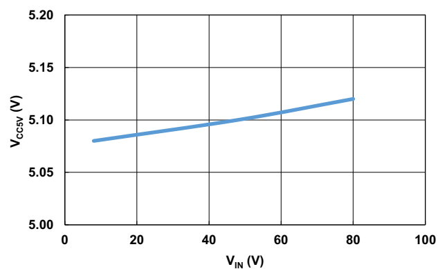
Figure 11. V CC5V Line Regulation at 20mA Load
