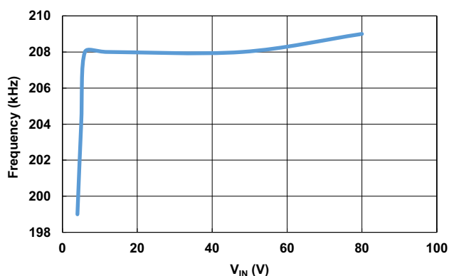
Figure 13. Switching Frequency vs V_{IN} , R_T = 169k
