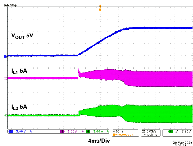
Figure 26. Dual-Phase Waveforms, Start-Up Waveform, V_{IN} = 48V I_O = 0A , CCM
