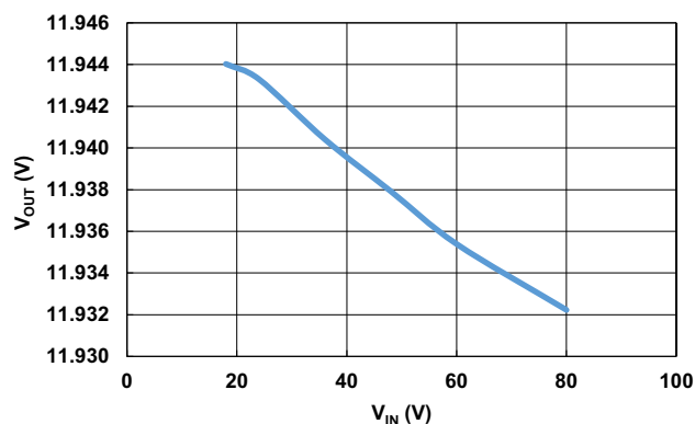
Figure 21. CCM Line Regulation at 20A Load +25°C
