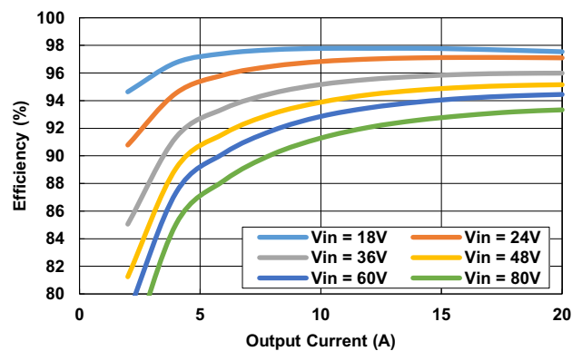
Figure 2. Efficiency ( V_{OUT} = 12V , CC Mode)
