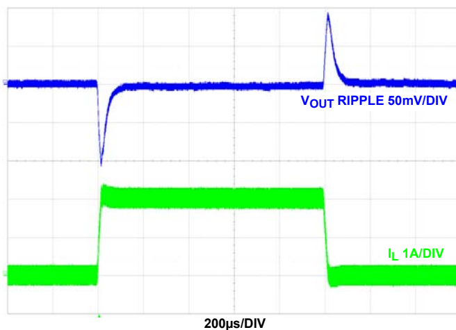
FIGURE 46. LOAD TRANSIENT F_{SW} = 2\text{MHz} , V_{IN} = 5\text{V} , \text{MODE} = \text{PWM} , T_A = +25^\circ\text{C}
