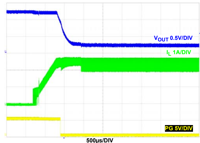
FIGURE 48. OVERCURRENT PROTECTION F_{SW} = 2\text{MHz} , V_{IN} = 5\text{V} , \text{MODE} = \text{PWM} , T_A = +25^\circ\text{C}
