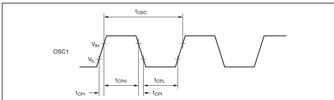
Figure 17.1 System Clock Input Timing
