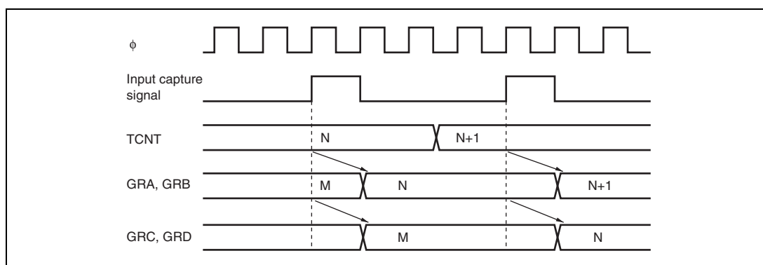
Figure 11.20 Buffer Operation Timing (Input Capture)
