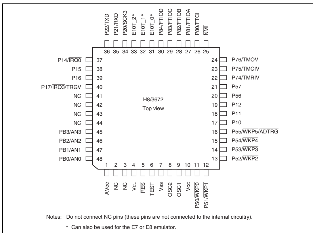
Figure 1.3 Pin Arrangement (FP-48F, FP-48B)
