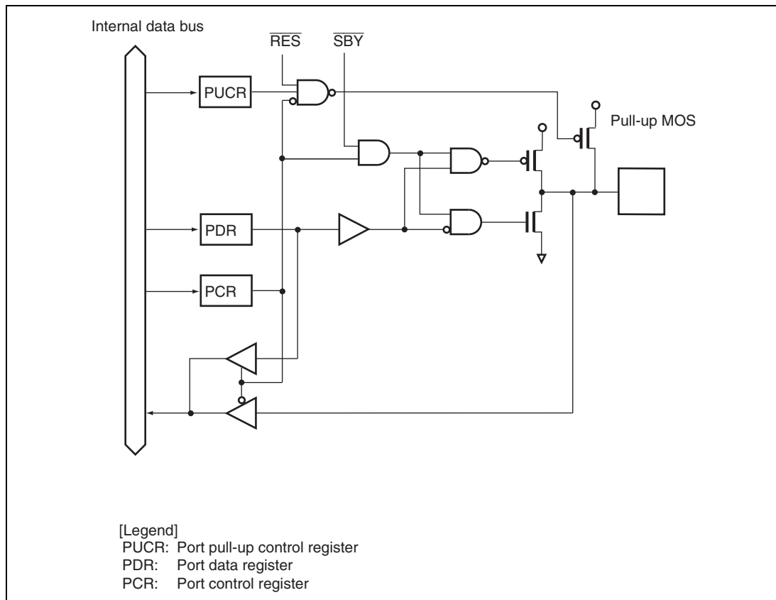
Figure B.4 Port 1 Block Diagram (P11)
