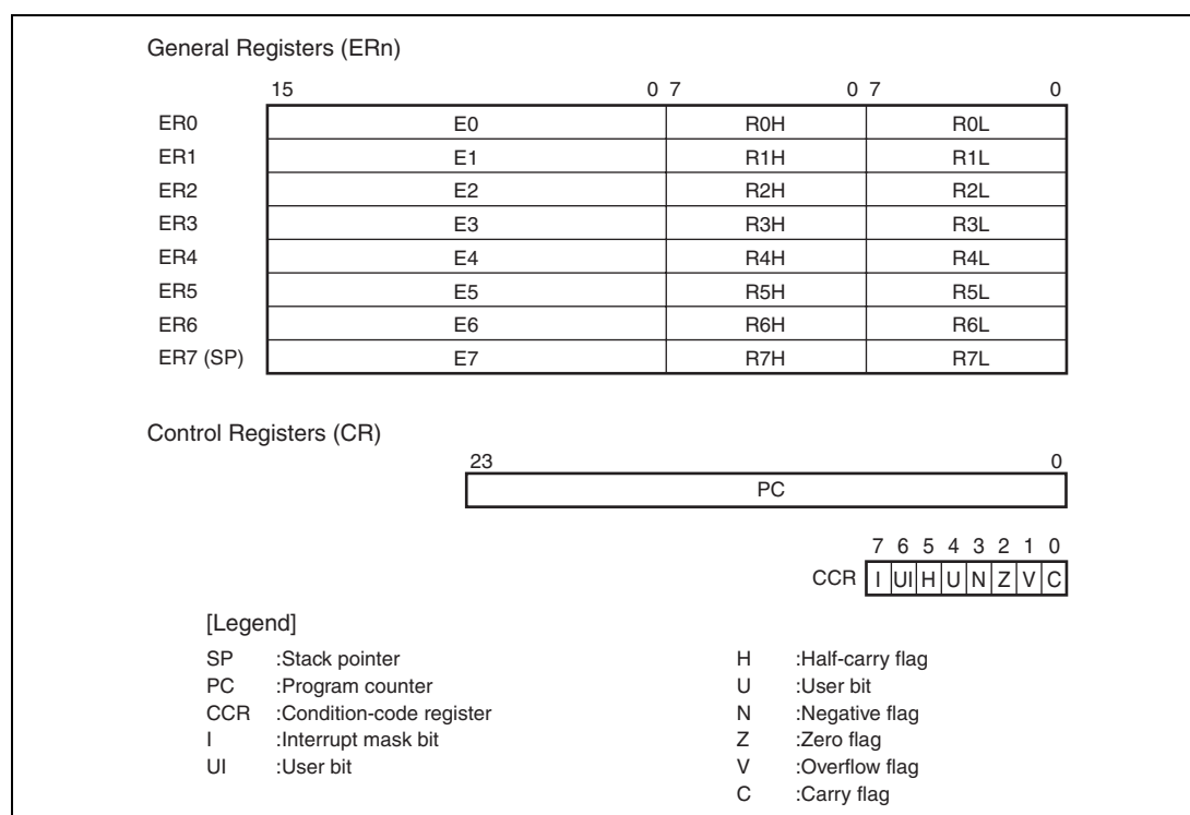
Figure 2.2 CPU Registers
