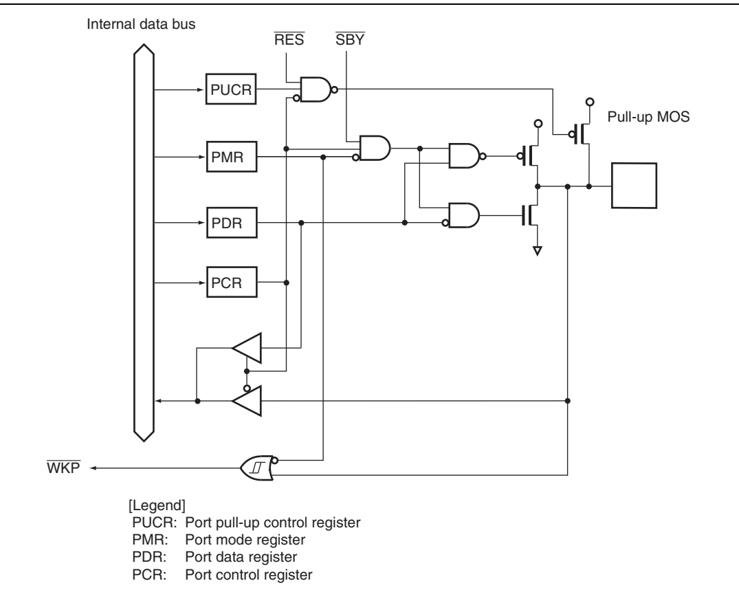
Figure B.10 Port 5 Block Diagram (P54 to P50)
