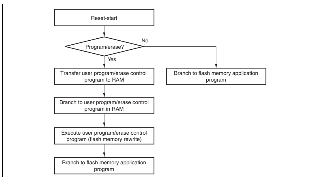
Figure 7.2 Programming/Erasing Flowchart Example in User Program Mode
