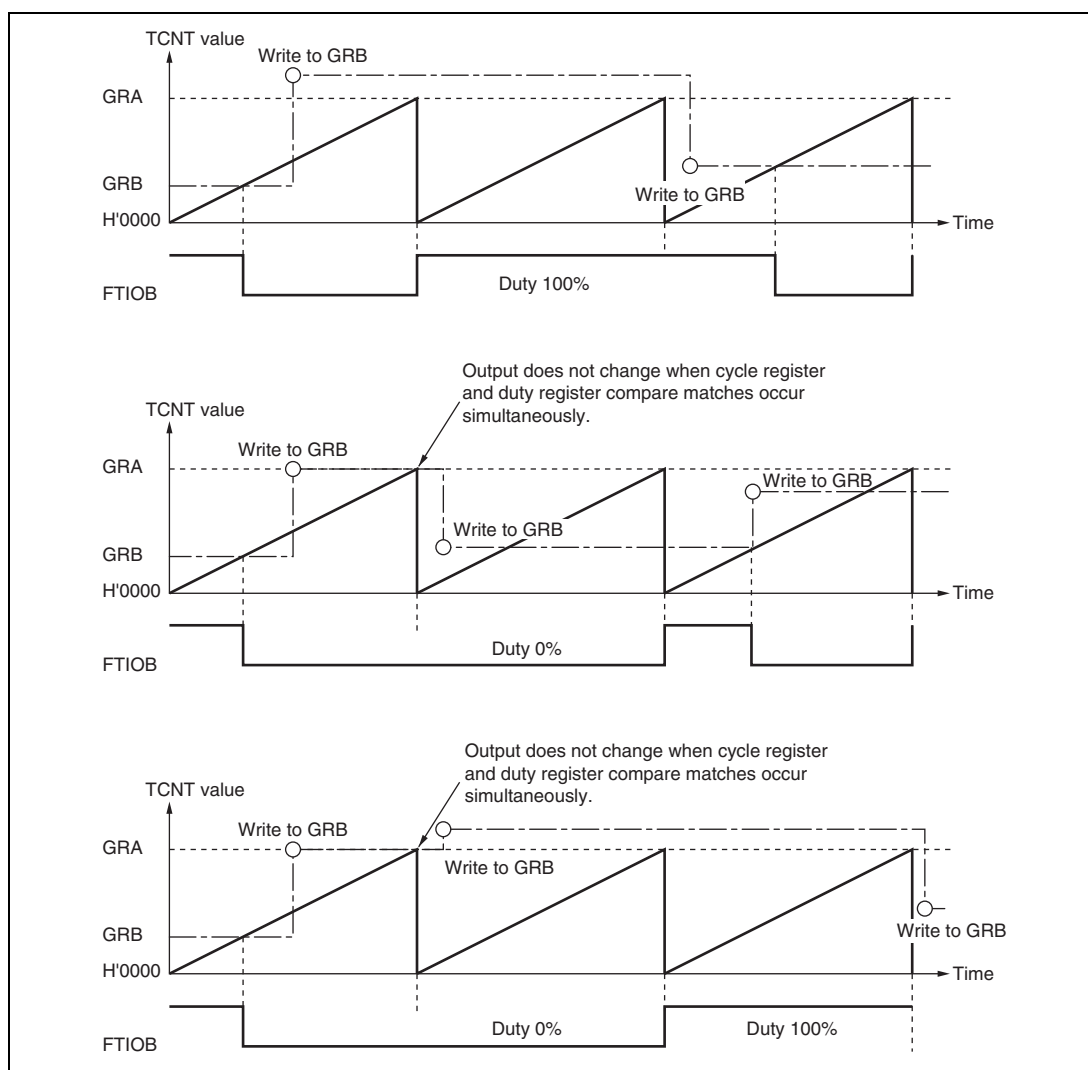
Figure 11.13 PWM Mode Example (TOB, TOC, and TOD = 1: initial output values are set to 1)
