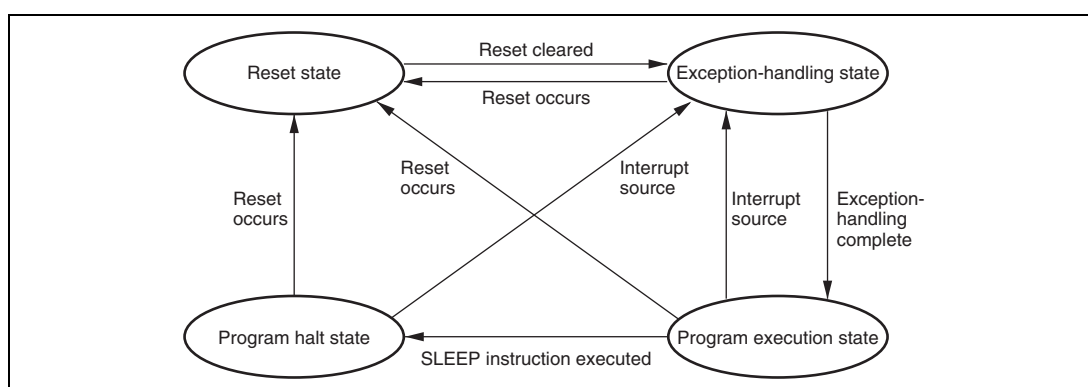
Figure 2.12 State Transitions
