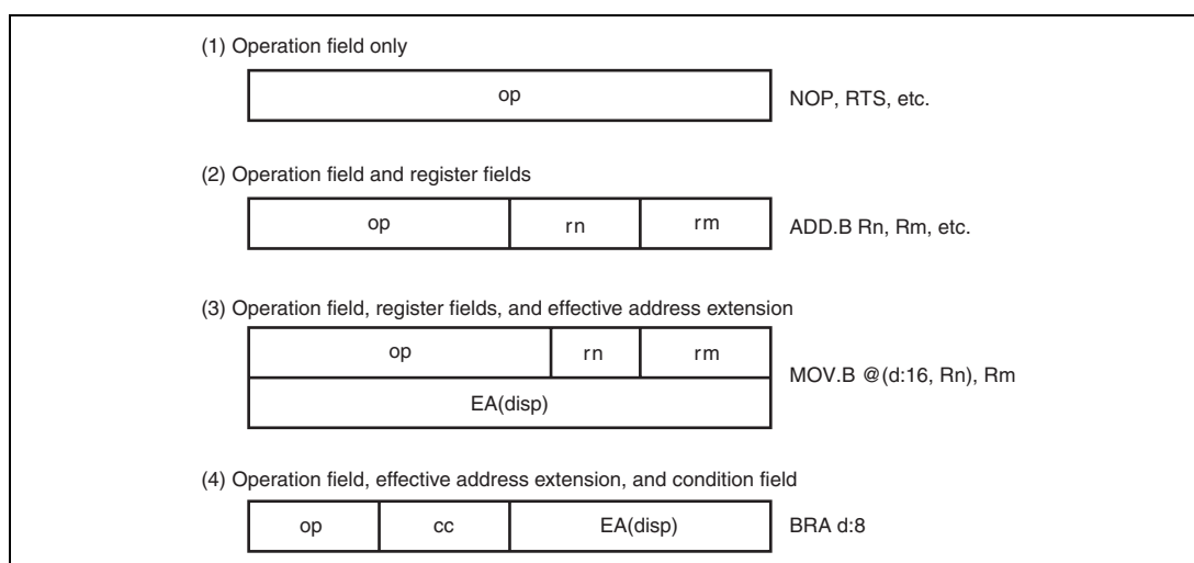
Figure 2.7 Instruction Formats
