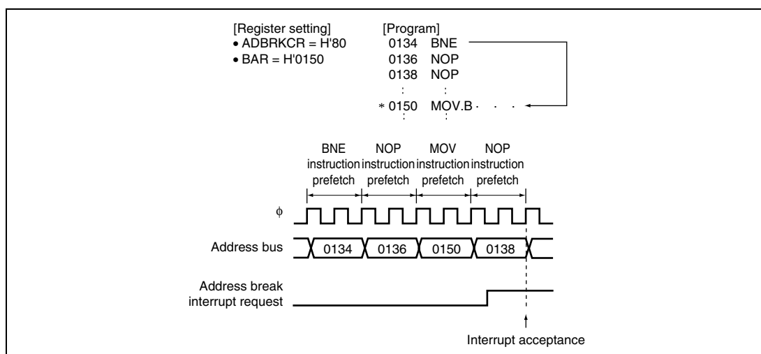
Figure 4.5 Operation when the Instruction Set is not Executed and does not Branch due to Conditions not Being Satisfied
