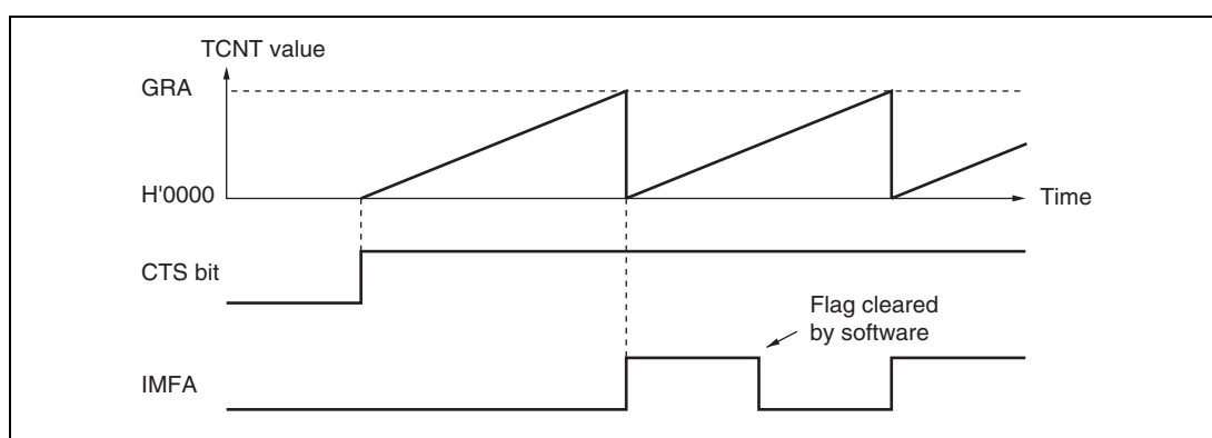
Figure 11.3 Periodic Counter Operation
