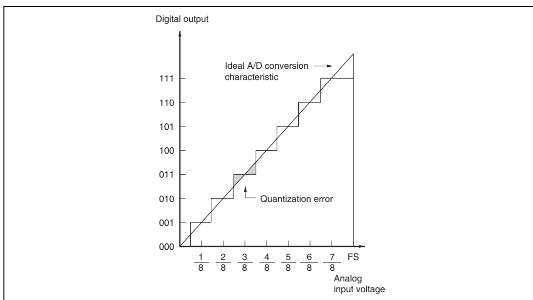
Figure 14.4 A/D Conversion Accuracy Definitions (1)
