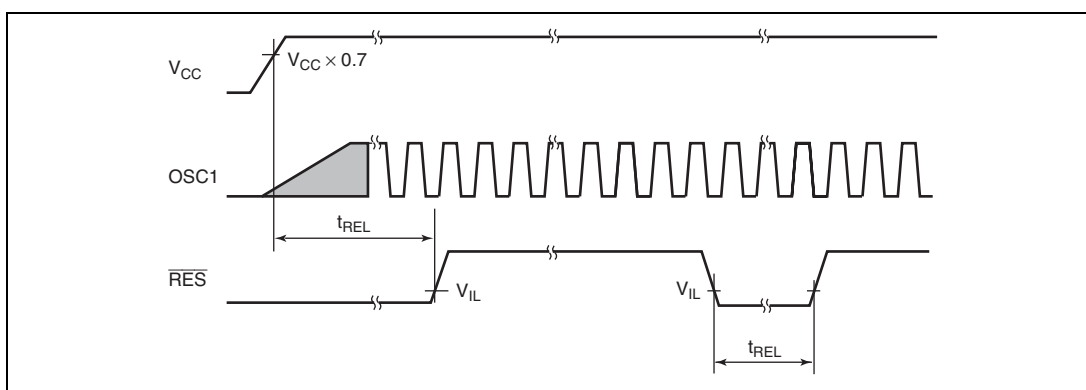
Figure 17.2 \overline{\text{RES}} Low Width Timing
