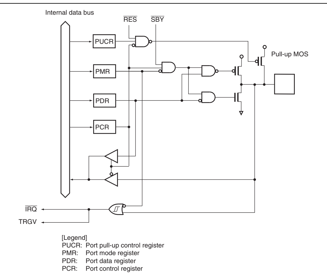
Figure B.1 Port 1 Block Diagram (P17)
