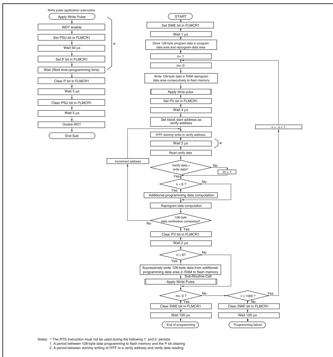
Figure 7.3 Program/Program-Verify Flowchart
