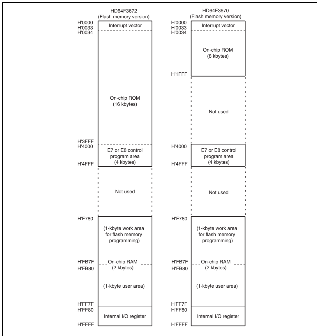
Figure 2.1 Memory Map
