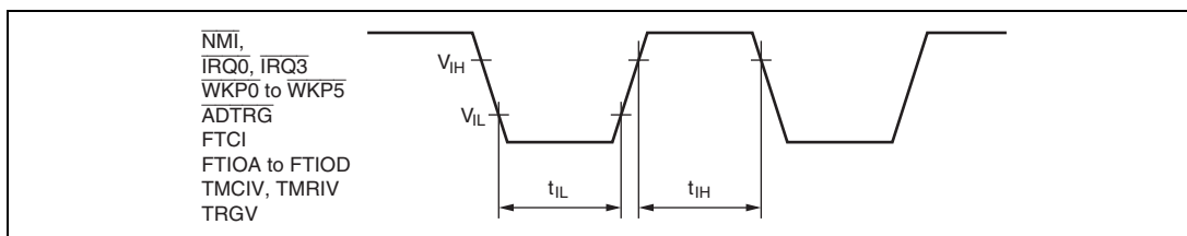
Figure 17.3 Input Timing
