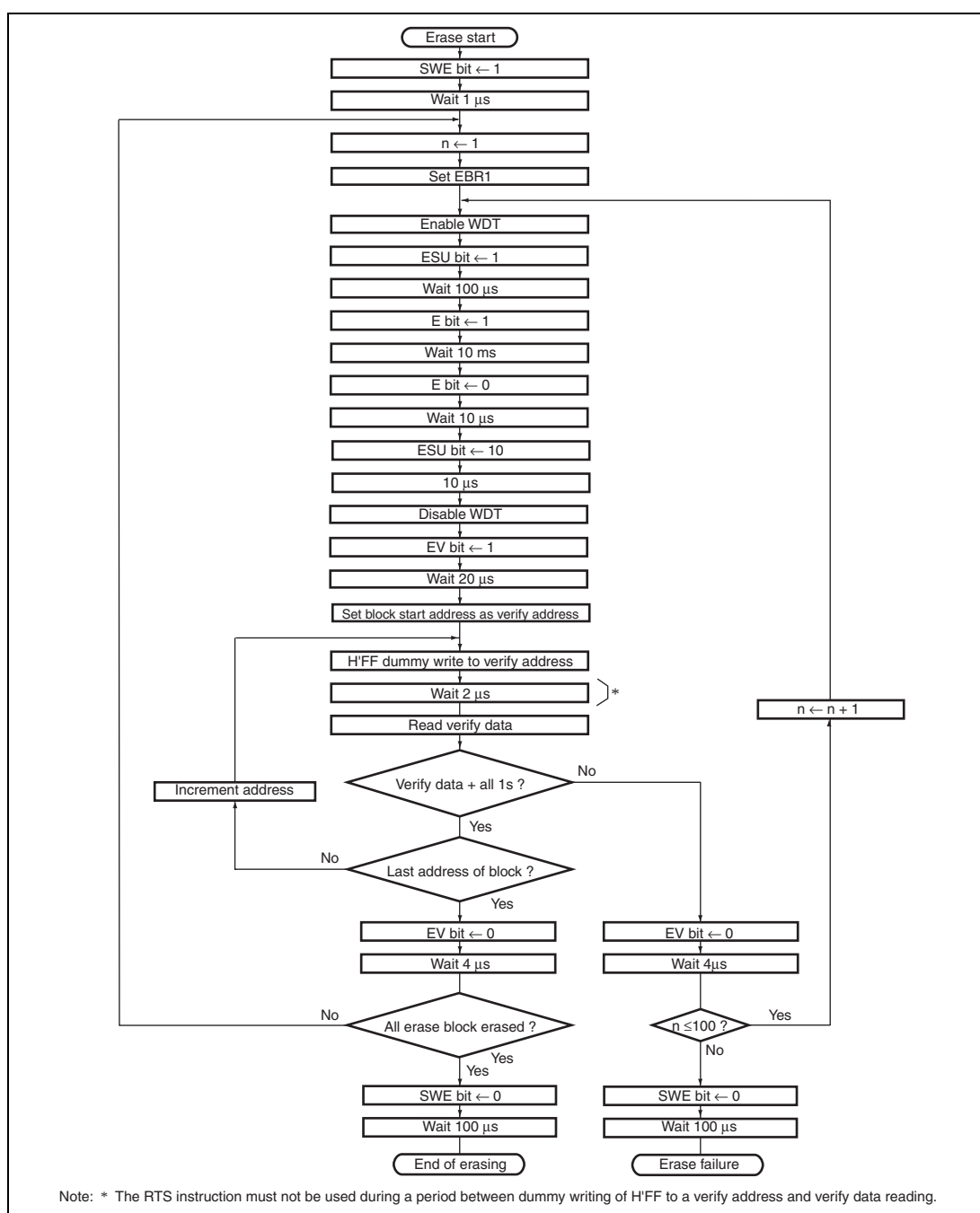
Figure 7.4 Erase/Erase-Verify Flowchart
