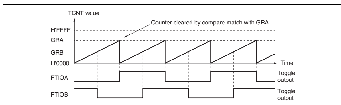
Figure 11.6 Toggle Output Example (TOA = 0, TOB = 1)
