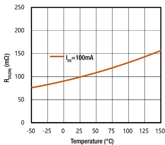
Fig. 4 R_{DS(ON)} vs Temperature
