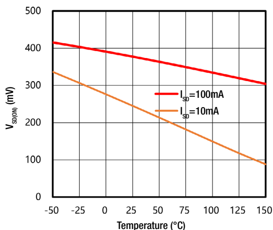
Fig. 3 V_{SD(ON)} vs Temperature
