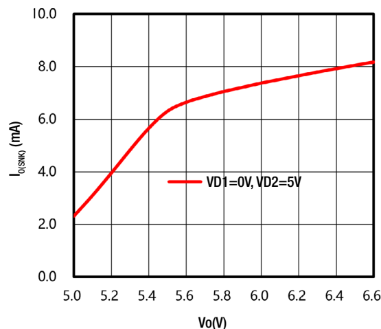
Fig. 2 I_{OS(NK)} vs V_O
