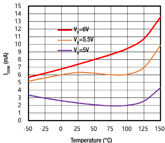
Fig. 1 I_{OS(NK)(MAX)} vs Temperature
