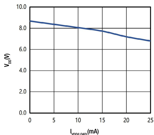
Fig. 8. V_{DD} vs I_{VDD(LOAD)}
