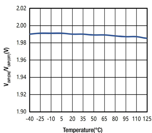
Fig. 6 V_{REF(REG)} vs Temperature
