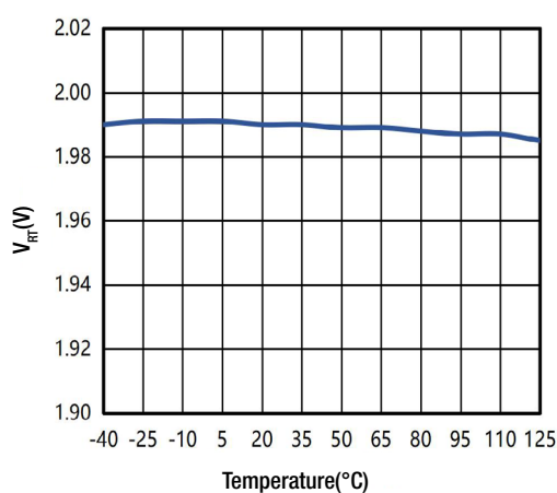
Fig. 3 V_{RT} vs Temperature
