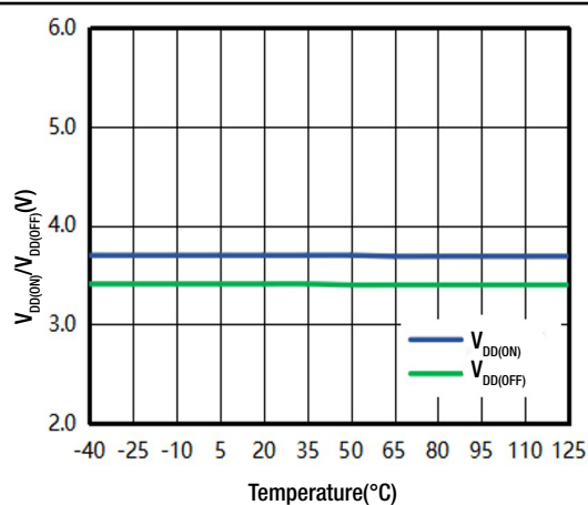
Fig. 4 V_{DD(ON)}/V_{DD(OFF)} vs Temperature
