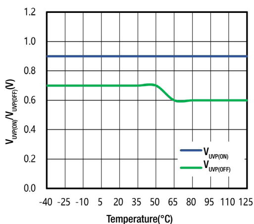
Fig. 5 V_{UMP(ON)}/V_{UMP(OFF)} vs Temperature
