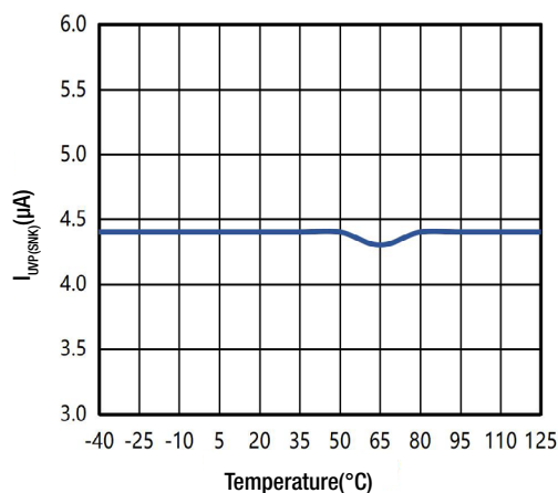
Fig. 1 I_{UMP(SNK)} vs Temperature
