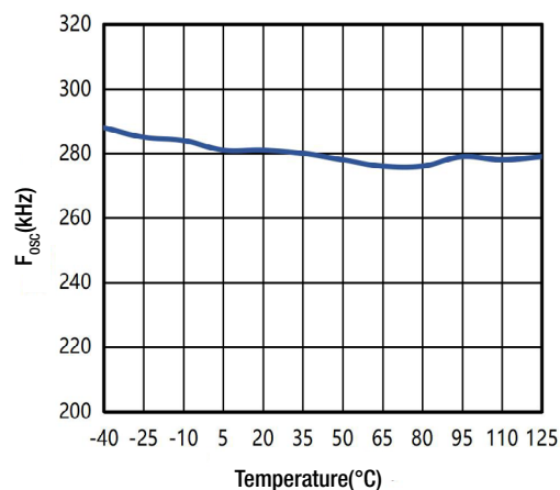
Fig. 2 F_{osc} vs Temperature @ R_T = 22k\Omega
