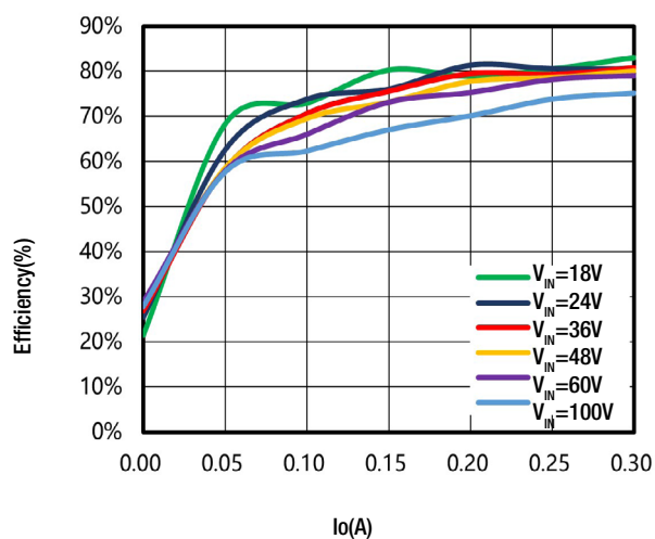
Fig. 22 Efficiency vs Io
