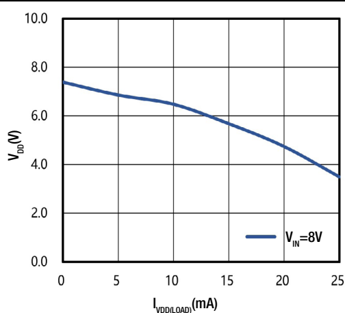
Fig. 9. V_{DD} vs I_{VDD(LOAD)}
