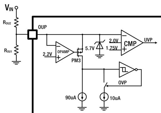
Fig. 17 Input Over/Under Voltage Protection
