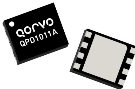
6 x 5 x 0.85mm DFN Package
