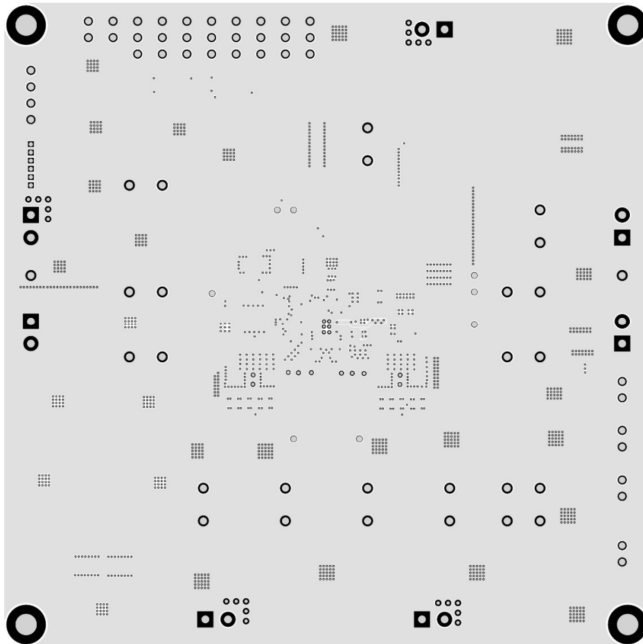
Figure 7 – Layout Layer 2
