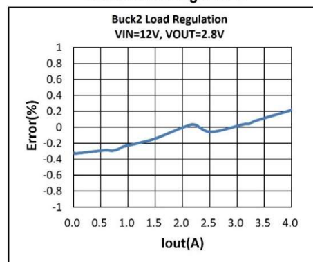
CMI 101 Buck2 Load Regulation
