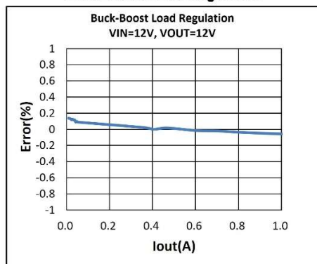
CMI 101 Buck-Boost Load Regulation
