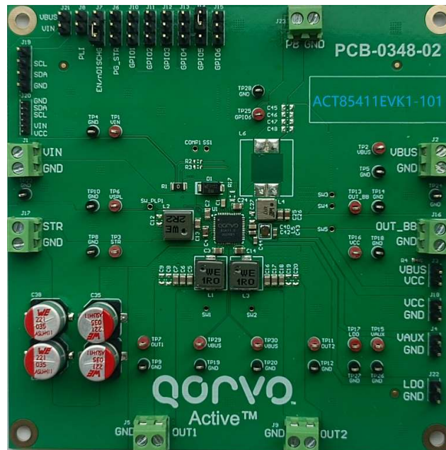
Figure 1 – EVK Picture
