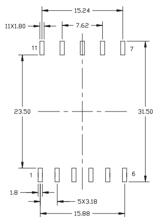
SUGGESTED LAND PATTERN
