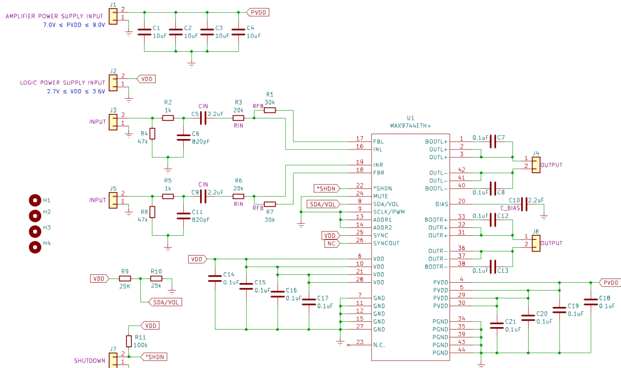
Figure 1. AMP2X2 schematic.
