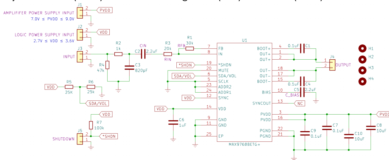
Figure 1. AMP1X2 schematic.
