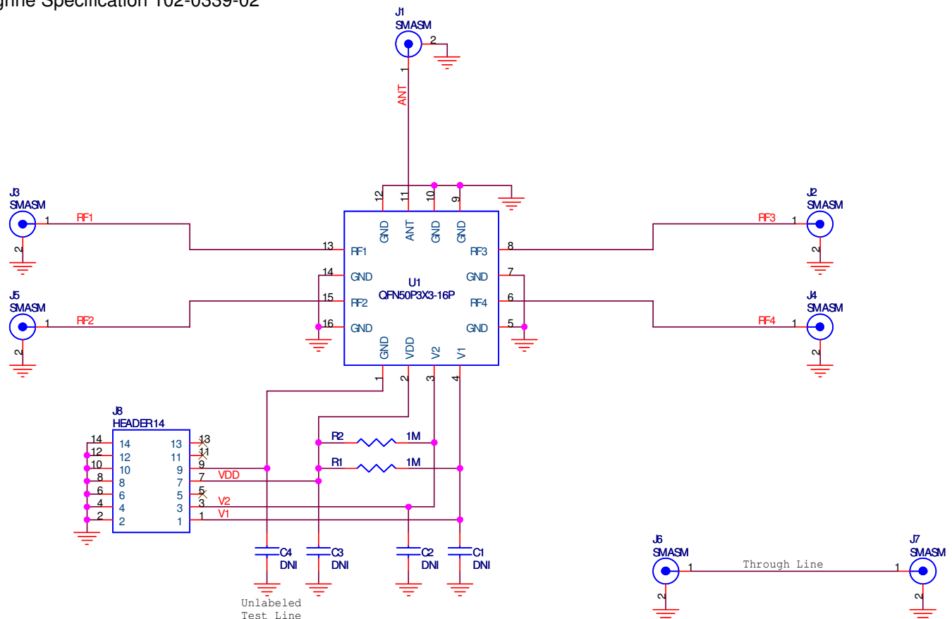
Figure 5. Evaluation Board Schematic
