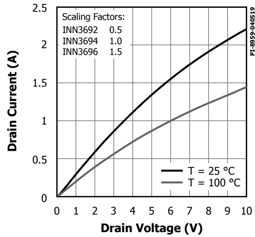
Figure 33. Output Characteristics.
