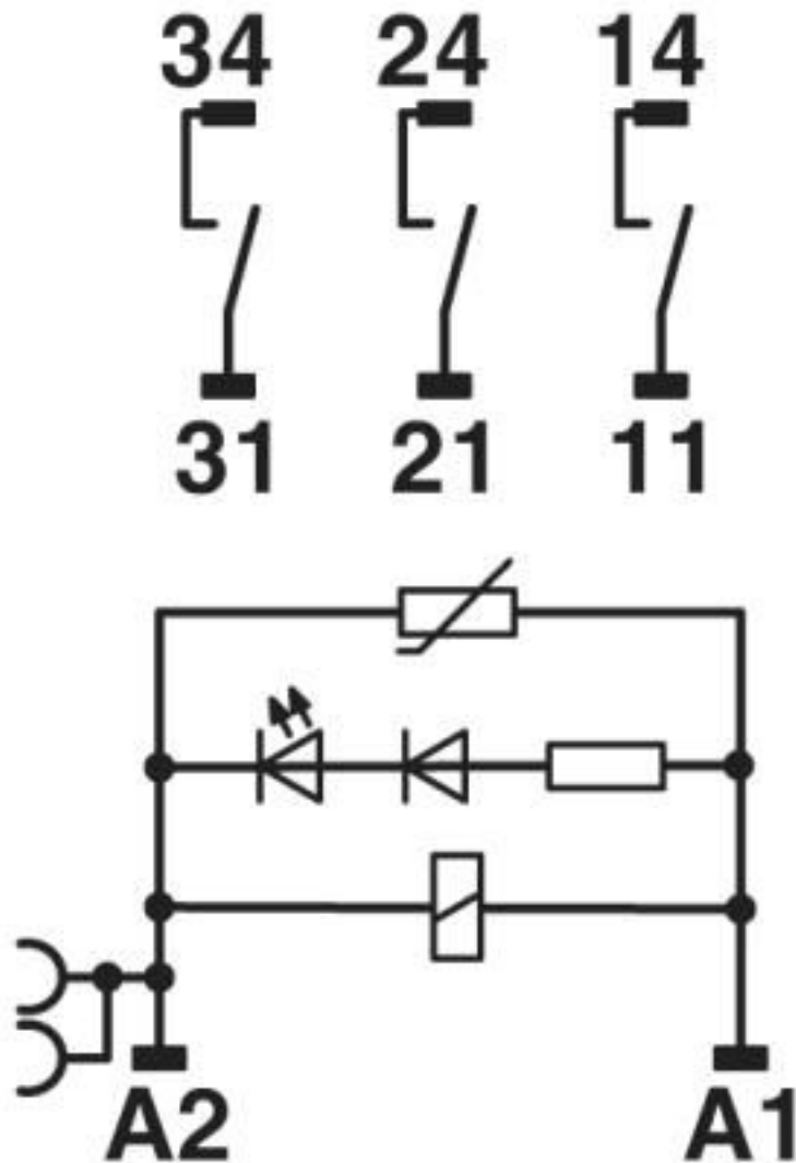
Circuit diagram
