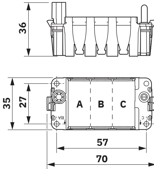
Dimensional drawing
