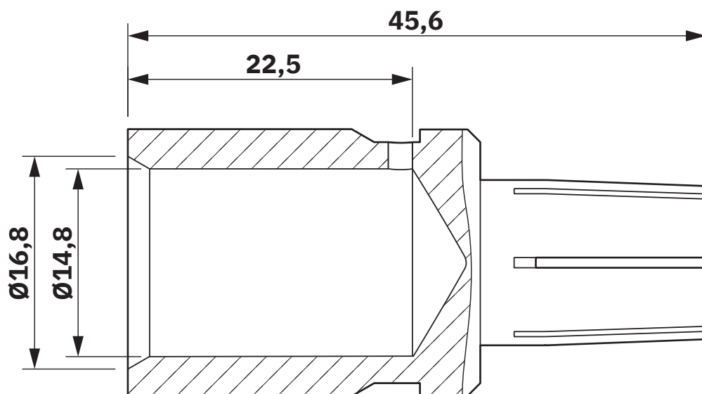
Dimensional drawing
