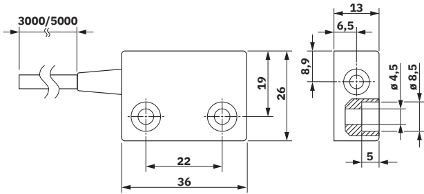
Dimensional drawing
