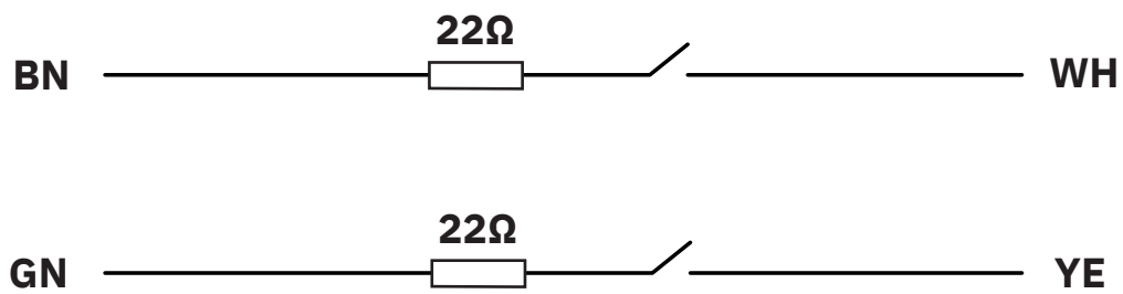
Circuit diagram
