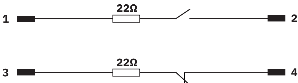
Circuit diagram
