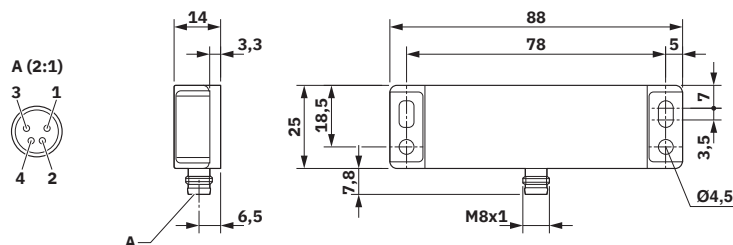
Dimensional drawing
