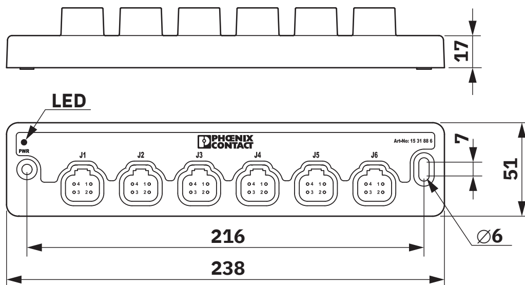
Dimensional drawing
