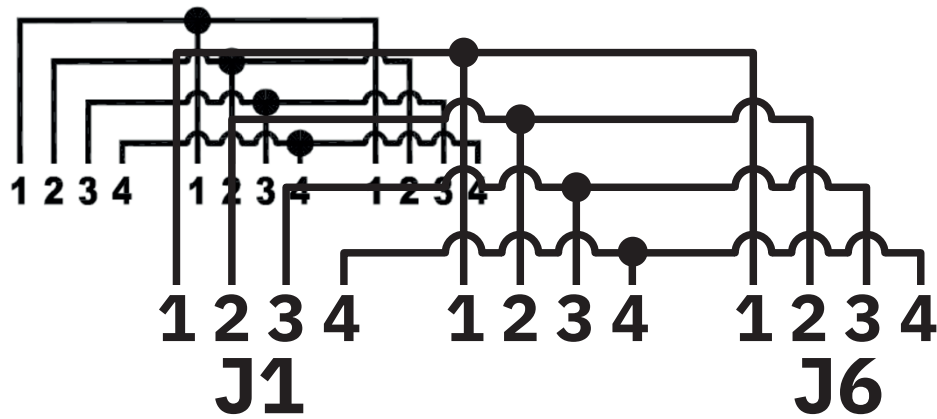
Circuit diagram
