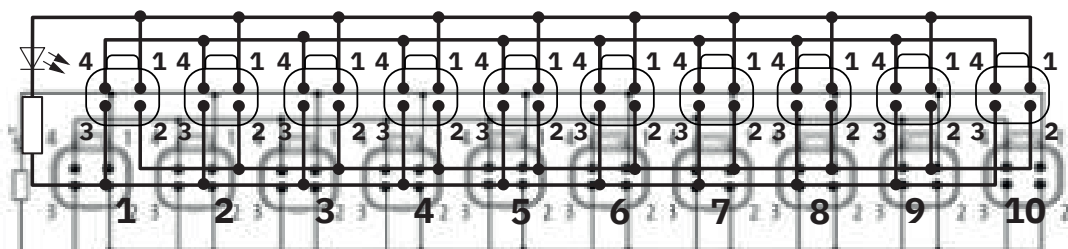
Circuit diagram
