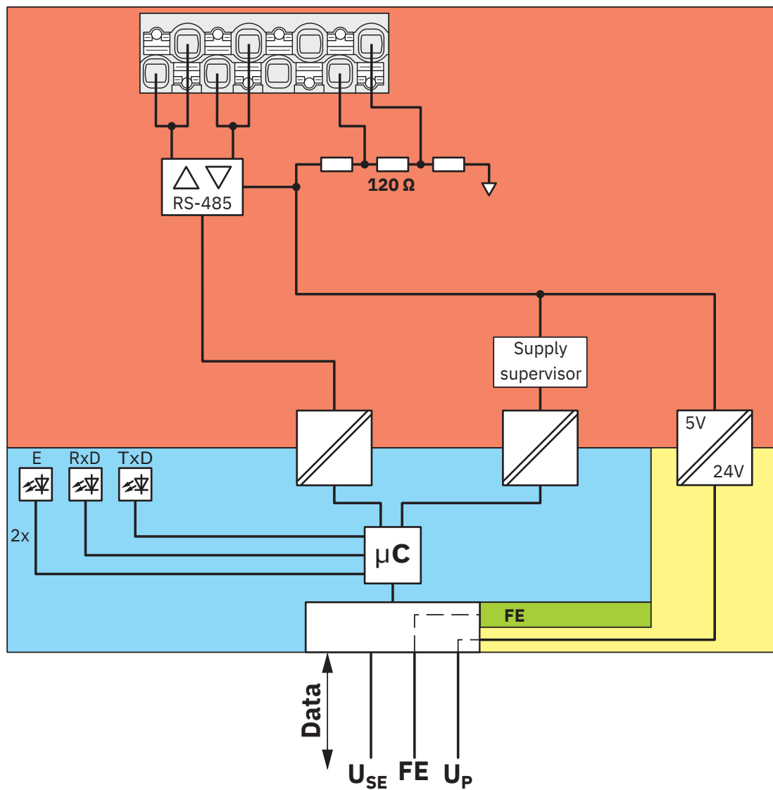
Block diagram
