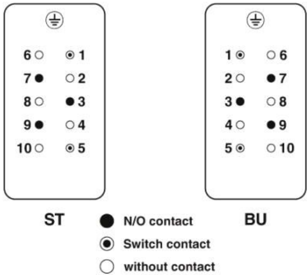
Schematic diagram
