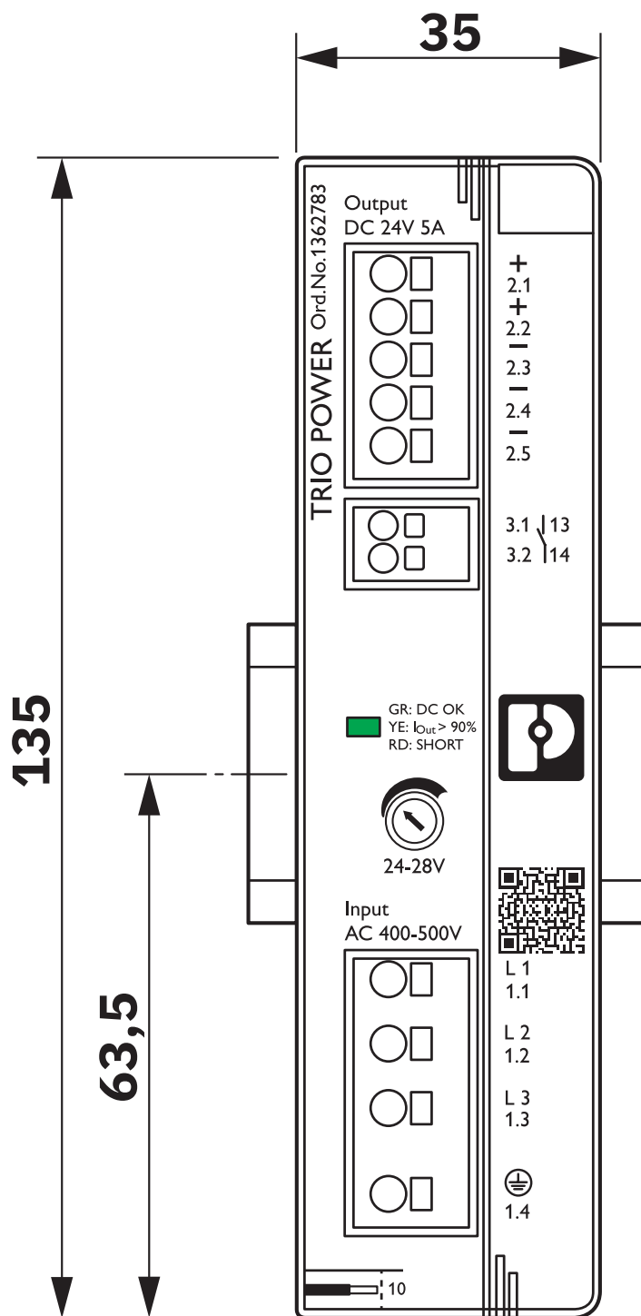
Dimensional drawing
