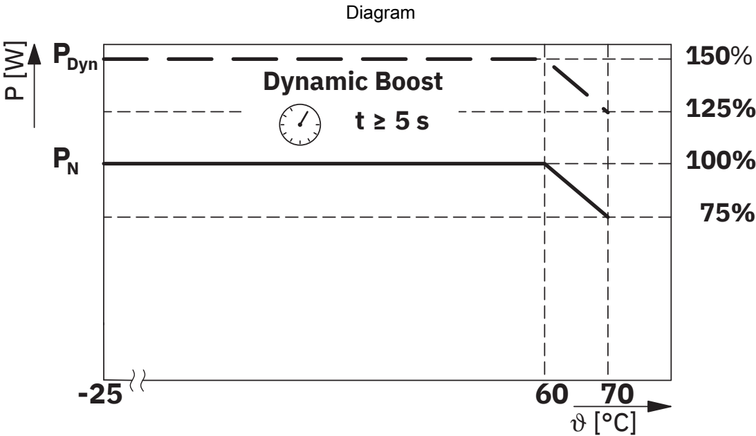
Temperature-dependent derating
